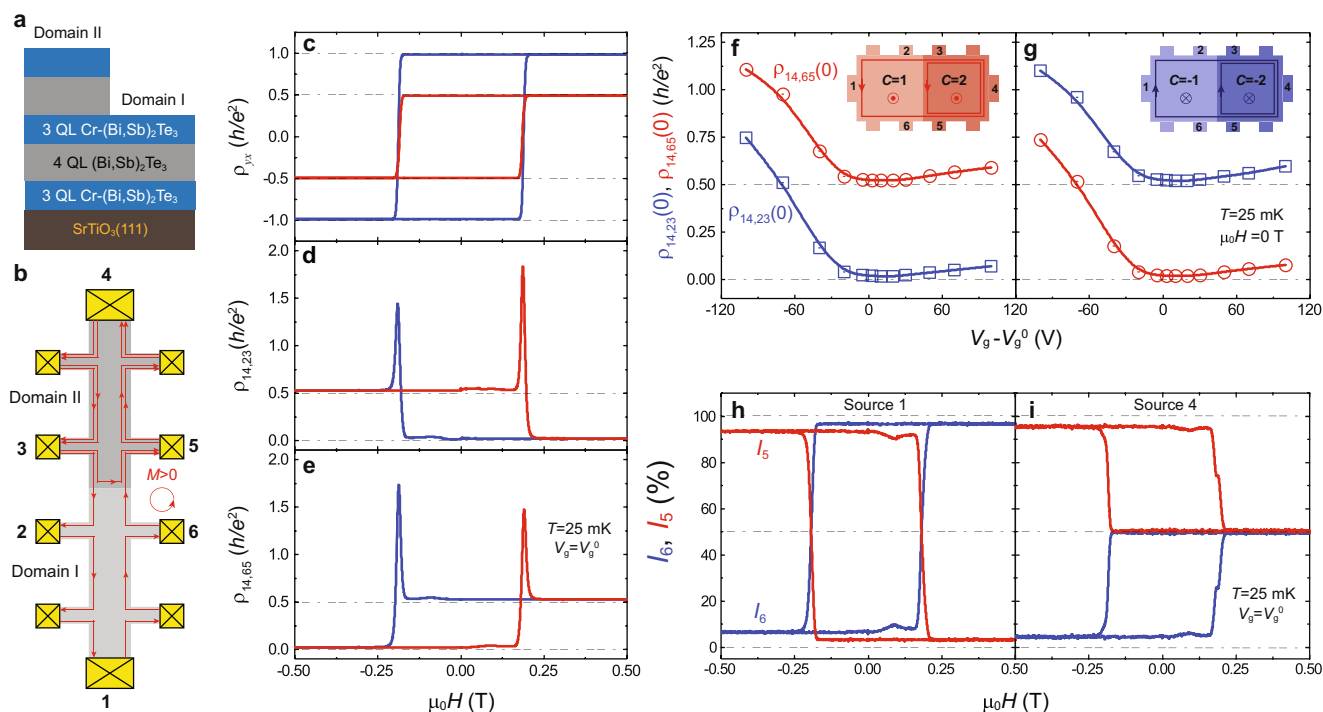
Fig. 4 | Creation of CICs along the junction between C=1 QAH and C=2 QAH insulators. a Side view of the magnetic TI multilayer structures for the junction between C=1 QAH and C=2 QAH insulators. b Schematic of the chiral edge/interface channels of the junction between C=1 QAH and C=2 QAH insulators for M > 0 . c \mu_0 H dependence of \rho_{xx} for Domain I ( C=1 , blue) and Domain II ( C=2 , red).
