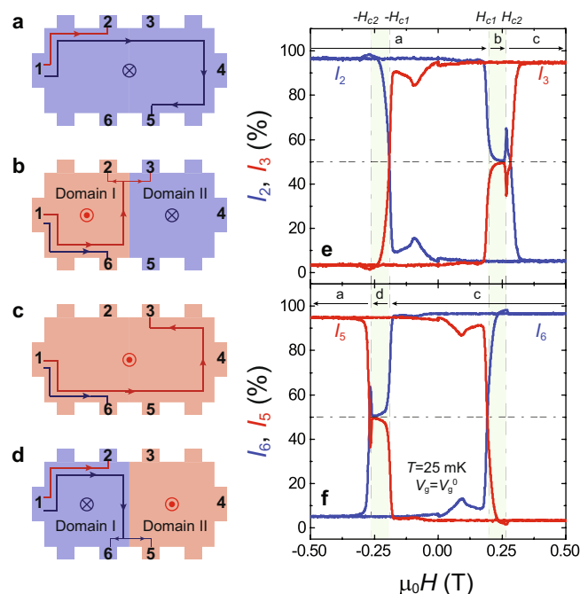
Fig. 3 | Chiral edge current distributor of the junction between C=1 QAH and C=-1 QAH insulators. a–d Schematics of chiral edge/interface current under different DW configurations, which are created by tuning external \mu_0 H . When a current of -1 nA is injected from contact 1, the drain current measured at contact 2 or 3 with other floating contacts is shown in red, while the drain current measured at contact 5 or 6 with other floating contacts is shown in blue. e \mu_0 H dependence of normalized drain current for contact 2 (blue) and 3 (red). f \mu_0 H dependence of normalized drain current for contact 5 (red) and 6 (blue). All measurements are performed at V_g = V_g^0 and T = 25 mK. The arrows in ( e , f ) indicate the magnetic field sweep directions and label the DW configurations in ( a–d ).
