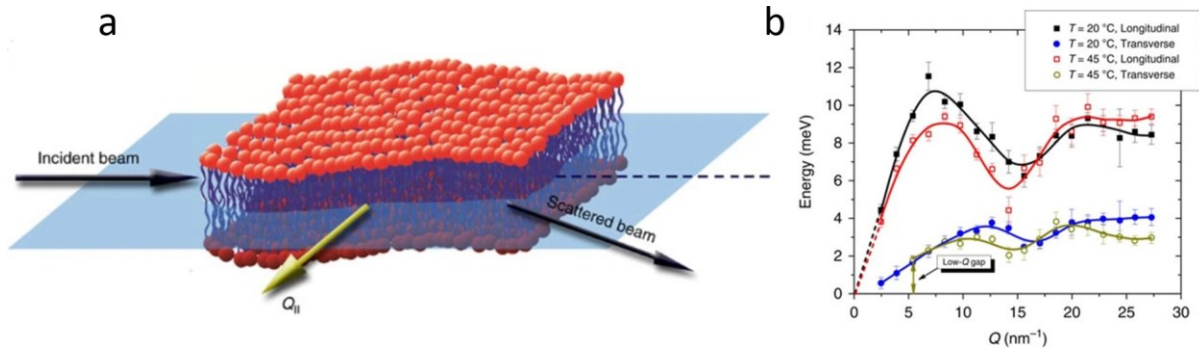
FIG. 5. E(Q) profiles of phonon dispersion relationships of a DPPC membrane in gel ( 20^\circ\text{C} ) and fluid ( 45^\circ\text{C} ) phases, respectively. The compelling experimental evidence of the phonon gap in the phospholipid membrane at low-energy and low-momentum values. Figure was adapted from Zhernenkov et al. (50).
