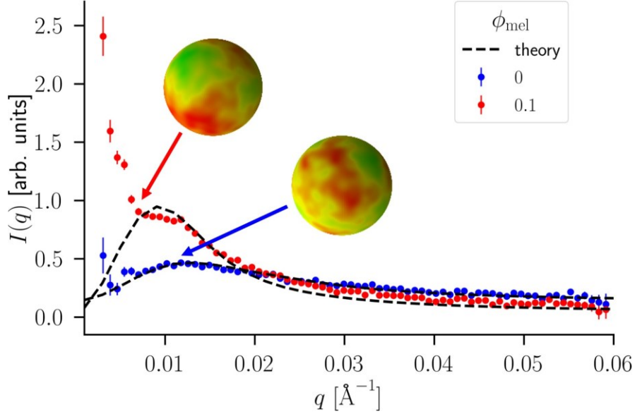
FIG. 4. Small-angle neutron scattering data from LUVs (50 nm in diameter) in the presence of 10% melatonin (red points) and in the absence of melatonin (blue points), reproduced from Ref. (45). The black dashed lines are fits to scattering data based on predictions from the theory related to the microemulsion phase (see Eq. (5)) taking into account the scattering signal from the lipids. Note that the addition of melatonin is consistent with the lipid raft formation of larger size as the scattering intensity peak shifts to smaller q values and becomes more prominent for \phi_{mel} = 0.1 .
