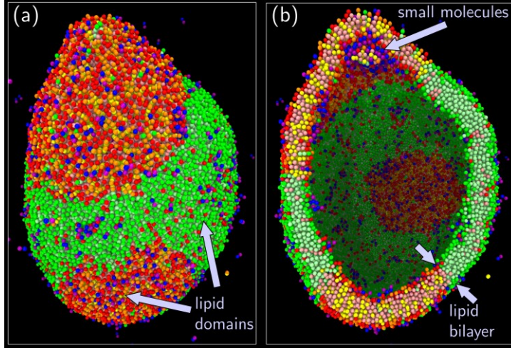
FIG. 3. Simulated lipid vesicle image (adapted from Ref. (42)) showing liquid ordered and liquid disordered domains (green/yellow versus red/orange regions) on the surface (a) and in a cross section (b). The data is obtained via high throughput molecular dynamics simulations, and more details are given in Ref. (42). The blue/purple particles represent small molecules which preferentially interact with the red/orange lipid phase. Note that the small molecules may aggregate and locally deform the membrane generating a spontaneous curvature (top region in (a) and (b)). Such preferential partitioning and membrane curvature generation are possible ways in which melatonin may influence the cell membrane properties and functions.
