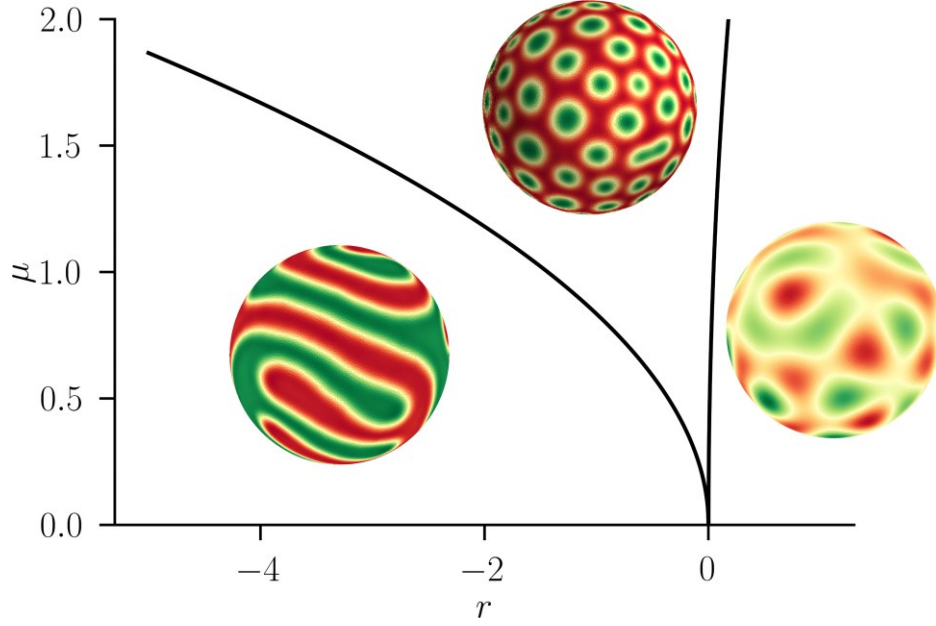
FIG. 2. Phase diagram for a fixed \kappa < 0 for the free energy given in Eq. 1. We find three different phases corresponding to striped patterns (left), hexagonal domain arrangements (center), and a microemulsion (right). The phase boundaries are indicated with solid black lines. Note that the configurations shown are constructed by evolving the dynamical equation in Eq. (2) for a free energy F (see Eq. (1)) with the given parameters. The dynamical equation is solved using the FiPy finite volume solver Python package (39).
