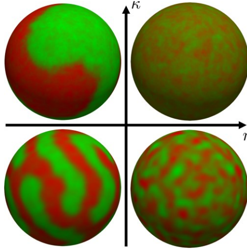
FIG. 1. Simulated lipid vesicles with free energies given by Eq. (1) with \mu = 0 and fixed signs of \kappa and r as shown. When \kappa, r > 0 (top right sphere), we find a homogeneous fluid phase, representing a mixed state of lipids. When \kappa > 0 and r < 0 (top left), the vesicle phase-separates into two distinct lipid phases (red and green), corresponding to liquid-ordered and liquid-disordered lipid regions. For \kappa < 0 , we find states with a characteristic length scale \lambda \approx \frac{2\sqrt{2}\pi}{\sqrt{-\kappa}} . For r > 0 , we find a disordered phase called a “microemulsion,” and it is thought to capture the properties of nanoscopic lipid heterogeneities in biological membranes (bottom right). Conversely, when r < 0 , we find a phase-separated, patterned (spatially modulated) phase (bottom left). These patterns may be striped, as shown, or have hexagonal arrangements of domains when \mu \neq 0 . All the lipid phase configurations are numerically generated by solving the dynamical equation Eq. (2) by using the FiPy finite volume solver Python package (39).
