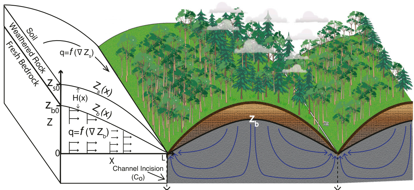
Fig. 1. Conceptual model showing the elevation of fresh bedrock, Z_b , under ridge and valley topography with a thin soil mantle overlying a weathered bedrock zone that extends to Z_b . Channel incision, at the rate C_0 , drives hillslope erosion and drainage of fresh bedrock (flow paths illustrated with blue arrows). (Left) The model framework and assumptions. At the ridgetop ( x = 0 ), the surface elevation is Z_{s0} and the fresh-bedrock elevation is Z_{b0} . Groundwater flux, q_w , is horizontal and proportional to the water table gradient, \nabla Z_b . Soil transport, q_s , is proportional to the surface slope, \nabla Z_s . All soil and water leaves the hillslope at L where the hillslope meets the channel. At steady state, the rate of channel incision ( C_0 ) is equal to the uplift rate such that the ground surface, Z_s and surface of the fresh bedrock, Z_b , are stationary.
