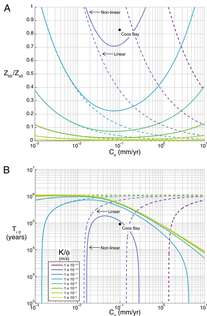
Fig. 3. Mapping the ratio of saturated hydraulic conductivity to porosity ( K/\phi ), fresh-bedrock relief ratio ( Z_{b0}/Z_{s0} ) and mean residence time ( T_{r0} ). (A) The influence of channel incision rate, C_o , on the fraction of the total hillslope relief that is unweathered ( Z_{b0}/Z_{s0} ). (B) The influence of C_o on the residence time of the weathered material that arrives at the soil-bedrock boundary at the ridgetop ( T_{r0} ). In both A and B, solid lines represent predictions using a nonlinear relationship between soil flux and slope (Eqs. S12 and S13) and dashed lines represent the linear model. Model parameters for Coos Bay were used to generate predictions (Table S1). A range of K/\phi is shown to illustrate how the deviation between the linear and nonlinear model predictions depend on K/\phi such that higher K/\phi will produce a thicker weathered zone. Deviations between the two model results are minimal at low C_o but increase with increasing C_o . Whereas the linear model predicts a thickening of the weathered zone (and thus an increase in residence time) with increasing erosion rate, the nonlinear model predicts a maximum weathered zone thickness that depends on the bulk density ratio, \rho_r/\rho_s , hillslope length, L , and critical slope, S_c .
