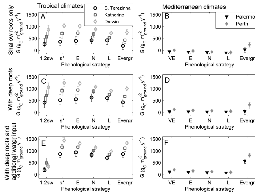
Figure 7. Median (symbols) and 25–75 percentiles (whiskers) of carbon gain G as a function of phenological strategy and access to deep water stores, for (left) three contrasting tropical climates and (right) two Mediterranean climates (Table I, Figure 1). A and B refer to plants with shallow roots ( \alpha=1 ). C–F refer to deep-rooted plants accessing the deep water store without ( I=0 ; C,D), or with groundwater recharge ( I=0.5 \text{ mm d}^{-1} ; E,F). Opportunistic flushing is triggered at s_{\text{flush}}=1.2s_w and s^* . Scheduled flushing is defined with respect to typical onset of wet season in tropical regions or the spring equinox in Mediterranean climates (VE, 40 days earlier; E, 20 day earlier; N, at the onset of wet season/equinox; L, 20 days after). All the other parameters are as in Figure 4. Additionally, for the carbon balance, f_{\text{resp}}=0.07 , f_c=0.45 , f_{\text{flush}}=1 \text{ y}^{-1} for drought-deciduous species and 0.67 \text{ y}^{-1} for evergreen species, \eta_A=0.65 , c_a=380 \mu\text{mol mol}^{-1} , a=1.6 , and A_{\text{max}} , g_{s,\text{max}} , and SLA are the median of the data in Figure 4 (only angiosperms are considered).
