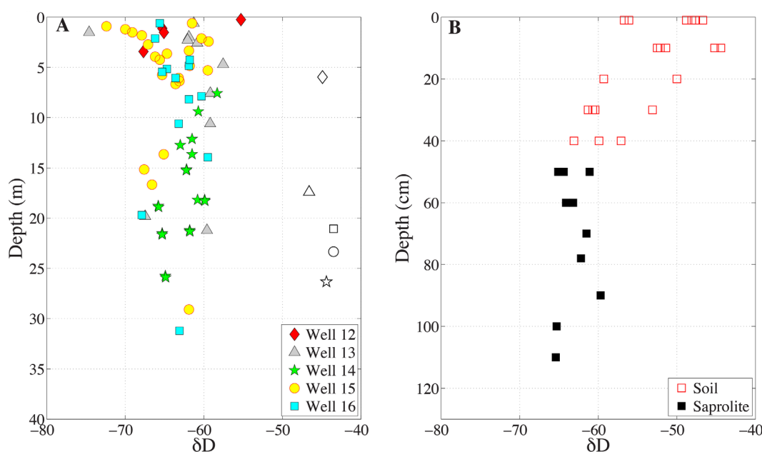
Figure 11. \delta D of bulk weathered bedrock as a function of depth below the surface. Samples taken during dry drilling and installation of 5 monitoring wells. Apart from well 12, the deepest sample at each well is in fresh bedrock, below Z b , and in the chronically saturated zone. Open symbols indicate the \delta D of groundwater at each well taken after drilling. Plot at right shows bulk \delta D through the soil and saprolite (collected with Kevin A. Simonin, published in Simonin et al. , [2014]).
