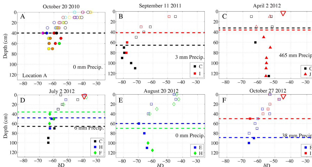
Figure 6. Bulk \delta D as a function of depth through the soil and saprolite at various sampling dates. Open symbols are soil, and closed symbols are saprolite. Date is indicated at the top of each plot. 20 October 2010 samples come from adjacent holes at site A (Figure 1). All other plots are from two to three locations from across hillslope with letter corresponding to location on Figure 2. Dashed horizontal lines (color coded for specific hole) indicate the depth of saprolite, and red triangle shows volumetrically weighted \delta D of previous rainfall (precipitation amount 30 days prior to sampling is included in each plot).
