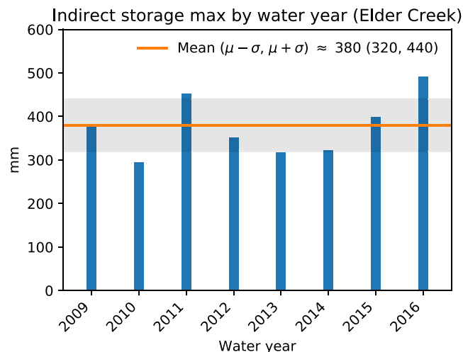
FIGURE 7 Maximum calculated indirect storage ( S_i ) at Elder Creek (with the grey envelope representing the mean plus or minus one standard deviation) for water years 2009–2016
