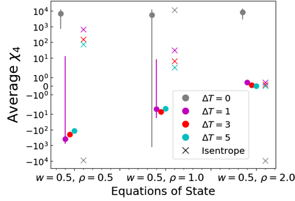
FIG. 12. Average \chi_4 across all hydrodynamic trajectories for the shifted freeze-out window.
