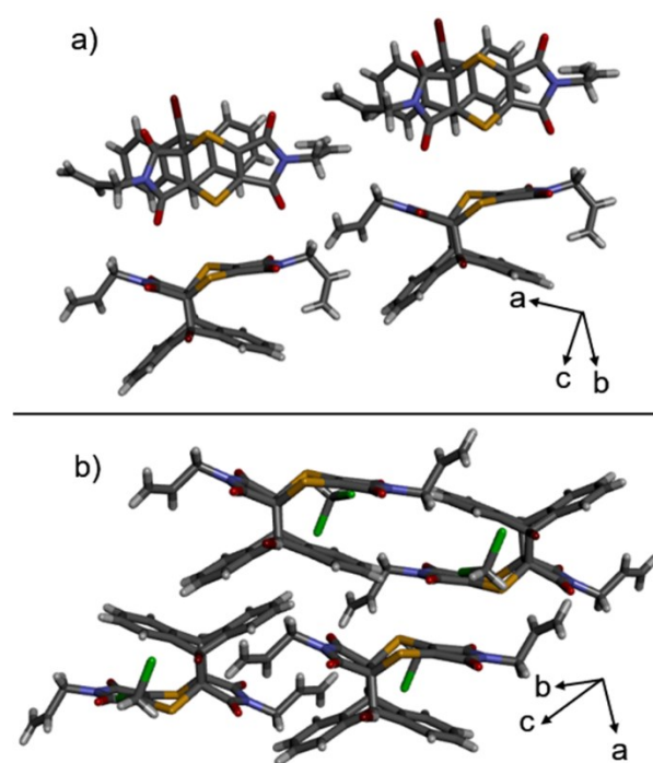
Figure 3. X-ray crystal structures of the CAs: a) non-solvated and b) DCM solvate.
