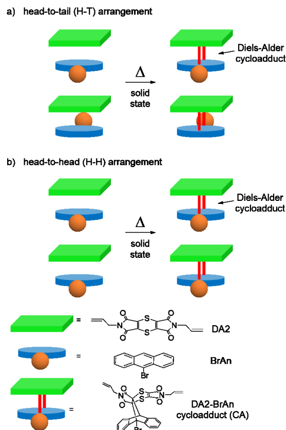
Scheme 1. Charge-transfer cocrystal polymorphs containing DA2 and BrAn arranged in a (a) H-T or (b) H-H geometry to undergo a Diels-Alder cycloaddition in the solid state.
