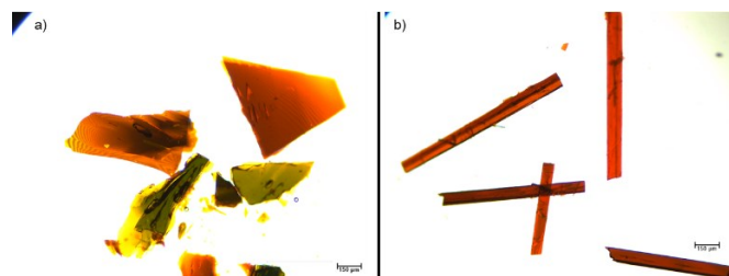
Figure 1. Polarized light microscopy images of the two DA2-BrAn polymorphs: a) large dichroic plates of the H-T polymorph and b) thin, elongated plates of the H-H polymorph.
