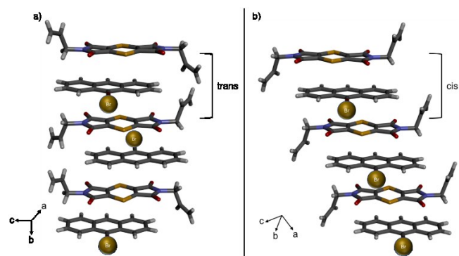
Figure 2. X-ray crystal structures of DA2-BrAn polymorphs: (a) H-T and (b) H-H highlighting \pi -stacking arrangement and positions of the bromine atoms and allyl groups.
