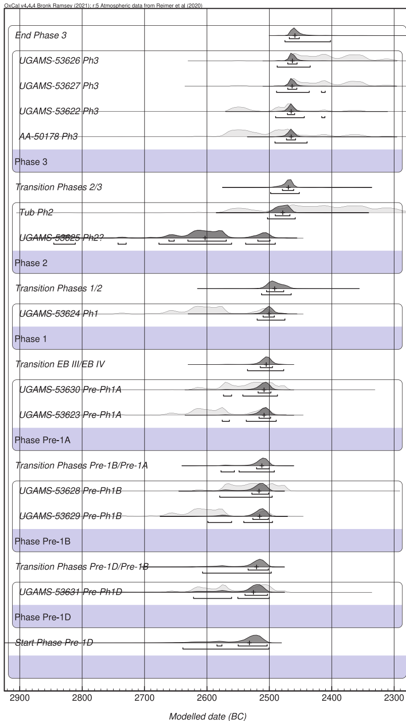
Figure 3 Bayesian model of AMS ^{14}\text{C} ages for seed and charcoal samples from Area C at Khirbat Iskandar, Jordan. Light gray curves indicate single-sample calibration distributions; dark curves indicate modeled calibration distributions. Calibration and Bayesian modeling based on OxCal v 4.4.4 (Bronk Ramsey 2009a) using the IntCal20 atmospheric curve (Reimer et al. 2020; van der Plicht et al. 2020). A_{\text{model}}=138.1 ; one statistical outlier: UGAMS-53625.
