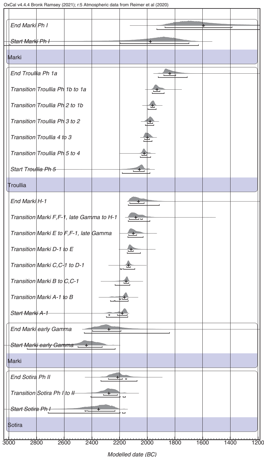
Figure 7 Bayesian sequencing of phase boundaries based on calibrated radiocarbon ages for seed and charcoal samples from Sotira Kaminoudhia , Marki Alonia and Politiko- Troullia , Cyprus; A_{\text{model}} = 182.5 . The dark curves indicate modeled calibration distributions. Calibrations and Bayesian modeling based on OxCal 4.4.4 (Bronk Ramsey 2009a) using the IntCal20 atmospheric curve (Reimer et al. 2020; van der Plicht et al. 2020).
