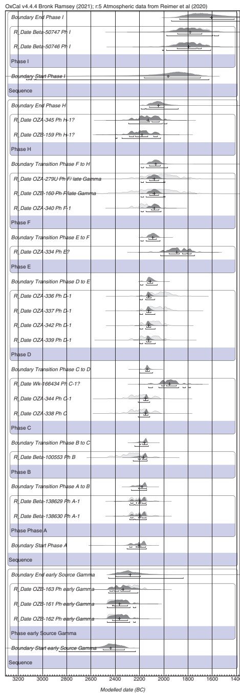
Figure 5 Bayesian sequencing of calibrated radiocarbon ages for 21 seed and charcoal samples from Marki Alonia, Cyprus; A_{\text{model}} = 154.7 . Light gray curves indicate single-sample calibration distributions; dark curves indicate modeled calibration distributions. Calibrations and Bayesian modeling based on OxCal 4.4.4 (Bronk Ramsey 2009a) using the IntCal20 atmospheric curve (Reimer et al. 2020; van der Plicht et al. 2020). Two samples (OZA-334 and Wk-166434) are excluded as statistical outliers based on A \leq 60 and two samples (OZA-345 and OZB-159) are excluded following Manning 2013b, Models 7–10.
