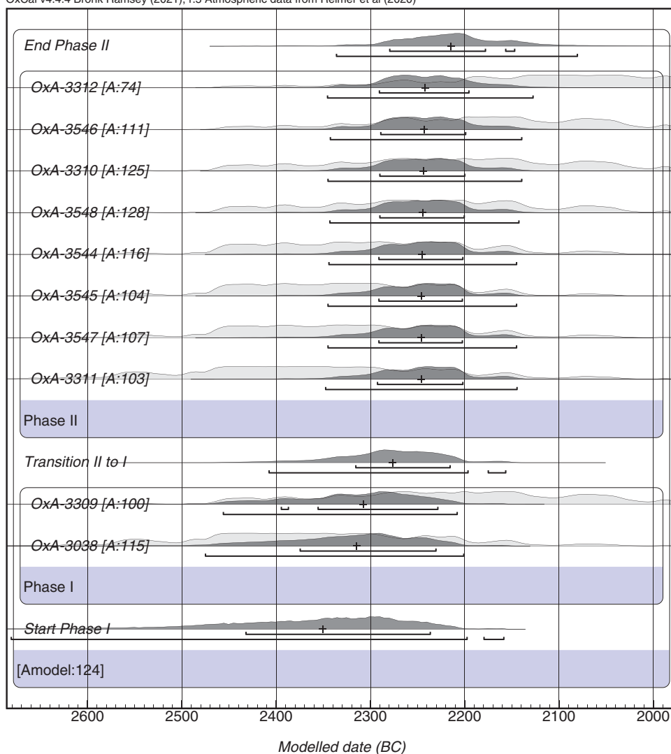
Figure 4 Bayesian sequencing of calibrated radiocarbon ages for 10 charcoal samples from Sotira Kaminoudhia , Cyprus; A_{\text{model}} = 124.0 . Light gray curves indicate single-sample calibration distributions; dark curves indicate modeled calibration distributions. Calibrations and Bayesian modeling based on OxCal 4.4.4 (Bronk Ramsey 2009a) using the IntCal20 atmospheric curve (Reimer et al. 2020; van der Plicht et al. 2020).
