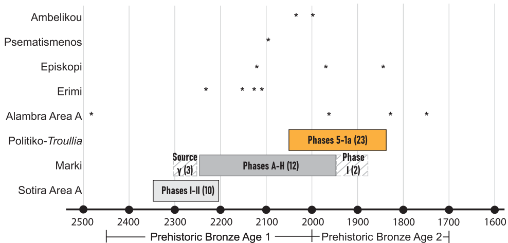
Figure 6 Schematic comparison of calibrated radiocarbon evidence from Prehistoric Bronze Age settlements on Cyprus. Bars depict Bayesian modeled sequences for calibrated radiocarbon ages from Politiko-Troullia, Sotira Kaminoudhia and Marki Alonia depicted according to modeled boundary medians (number of modeled ages for each sequence indicated in parentheses). Modeling of Troullia excludes two dates from Phases 3 and 2 that are statistical outliers. Marki excludes four ages: two from Phase H-1 and two statistical outliers (see Manning 2013b: table 1, figs. 7, 10). Radiocarbon ages from Alambra, Ambelikou, Episkopi, Erimi, and Psematismenos are plotted as individual unmodeled calibrated dates.
