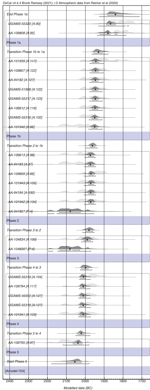
Figure 3 Model 1: Bayesian sequencing of calibrated radiocarbon ages for 25 seed and charcoal samples from Politiko-Troullia, Cyprus; A_{\text{model}} = 153.7 . Light gray curves indicate single-sample calibration distributions; dark gray curves indicate modeled calibration distributions. Calibrations and Bayesian modeling based on OxCal 4.4.4 (Bronk Ramsey 2009a) using the IntCal20 atmospheric curve (Reimer et al. 2020; van der Plicht et al. 2020). Two ages (AA-94185, AA-104835) are excluded as statistical outliers based on A \leq 60 .
