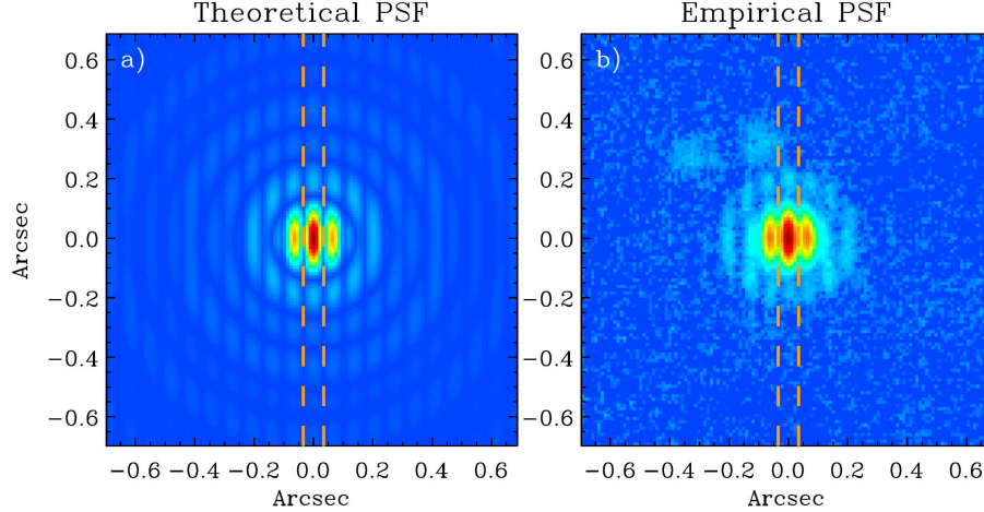
Figure 2. Theoretical (a) and observed (b) Fizeau PSF obtained with LBTI/LMIRCam 19 at 4.8\,\mu\text{m} . The vertical, dashed lines indicate the theoretical location of the first dark fringes. The two faint sources in the upper-left of the observed PSF are optical due to internal reflections in the instrument that have been mitigated since these data were taken.
