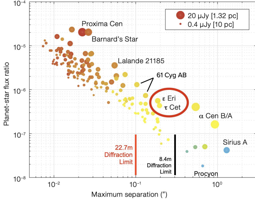
Figure 6. Separation, brightness, and contrast of a rocky, HZ planet around the nearest stars (tbd: what planet exactly, more details, additional points to highlight, reference?).
