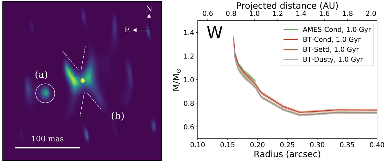
Figure 4. Recent LBTI interferometry results. Left : Model-independent image of the MWC 297 disk and companion candidate using fringe-tracked NRM observations 25 . Only \sim 10 min of science data were obtained to derive this image demonstrating the LBTI’s snapshot capabilities. Right : Contrast curves from Fizeau observations of Altair 29 obtained with LMIRCam reaching down to a separation of \sim 0.15 arcsec from the star, the strongest direct-imaging constraints on companions around that star available today at such small separations.
