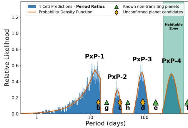
Figure 7. Probabilistic analysis of the known planets in the \tau Ceti system suggesting the presence of a super-Earth or mini-Neptune planet in the HZ 41 .
