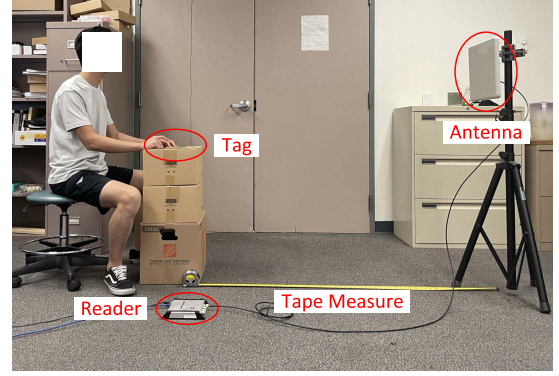
Fig. 17. Experiment setup.
