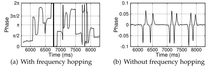
Fig. 7. Mitigating frequency hopping in phase data.
