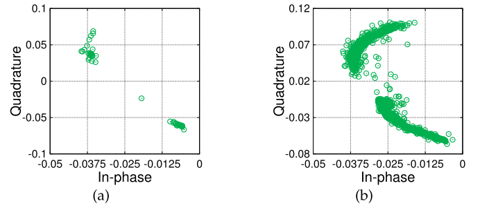
Fig. 15. (a) Extracted samples for phase recovery; (b) The adversary's sniffed symbols for Fig. 14(a).
