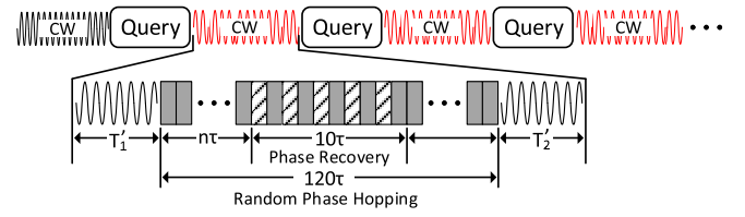
Fig. 13. Timing diagram of phase hopping.
