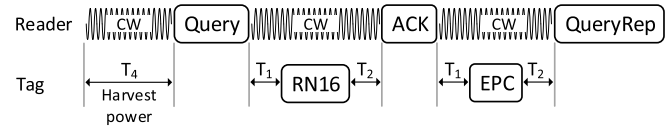
Fig. 2. The basic EPC Gen-2 query protocol with a single RFID card.
