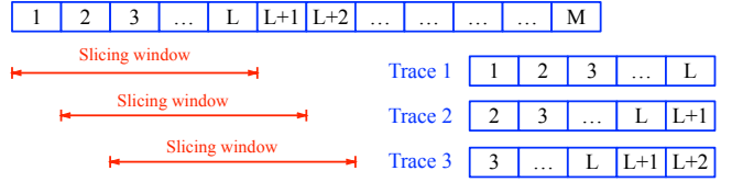
Slicing window with size L and stride 1
