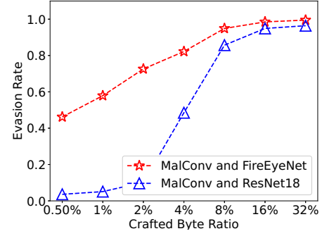
Fig. 10. Evasion rate of our method with different input formats.
