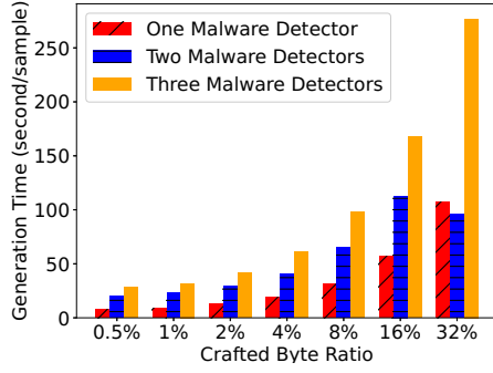
Fig. 9. Generation time of our method against different numbers of malware detectors.
