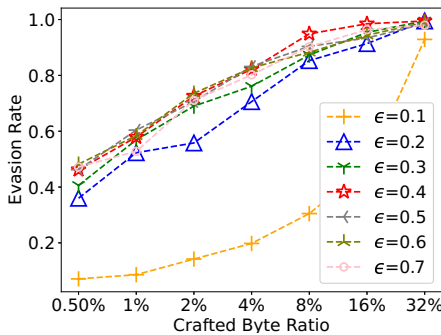
Fig. 3. Evasion rate of our method with different adversary strength \epsilon .
