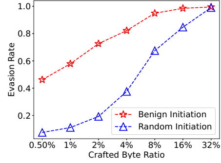
Fig. 8. Evasion rate of our method with different initialization approaches.
