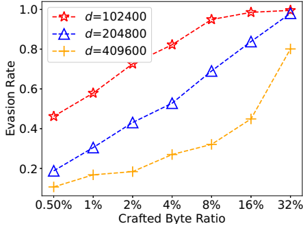
Fig. 6. Evasion rate of our method with different input size d .
