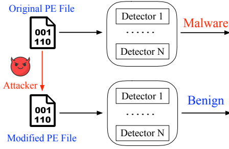
Fig. 1. Evasion Attacks against Multiple Malware Detectors.
