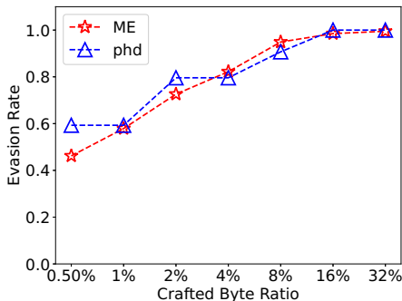
Fig. 7. Evasion rate of our method over different datasets.
