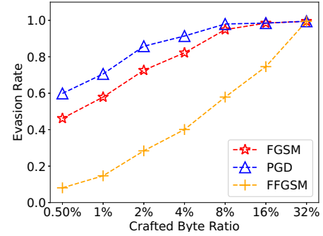
Fig. 4. Evasion rate of our method with different gradient-based algorithms.
