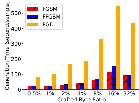
Fig. 5. Generation time of crafted programs in our method with different gradient-based algorithms.
