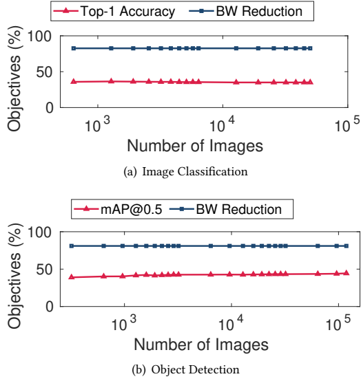
Figure 7: Objectives vs. The Sampling Size.
