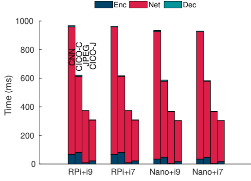
Figure 15: End-to-end image processing and networking latency breakdown over LTE (DET).
