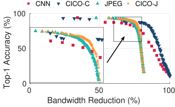
Figure 9: Accuracy-bandwidth trade-offs (CLS).
