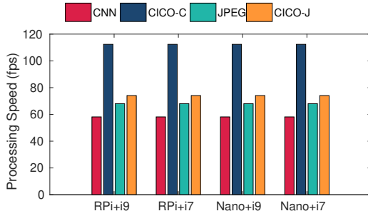
Figure 16: End-to-end image processing rate over WiFi (CLS).
