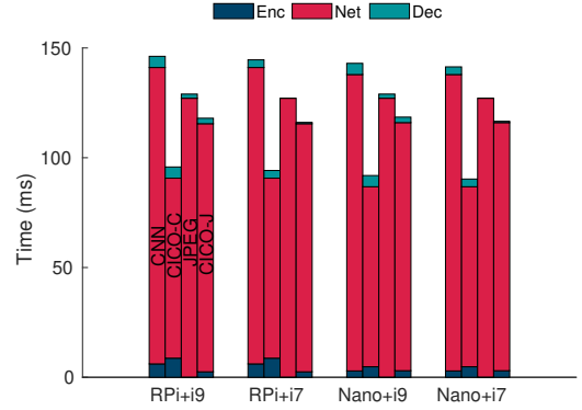
Figure 13: End-to-end image processing and networking latency breakdown over LTE (CLS).
