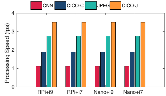
Figure 19: End-to-end image processing rate over LTE (DET).
