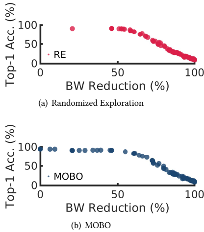
Figure 6: Explored configurations by RE and MOBO.
