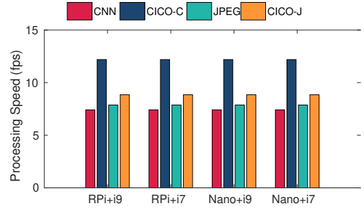
Figure 17: End-to-end image processing rate over LTE (CLS).
