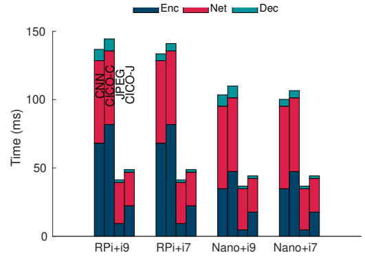
Figure 14: End-to-end image processing and networking latency breakdown over WiFi (DET).
