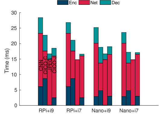
Figure 12: End-to-end image processing and networking latency breakdown over WiFi (CLS).
