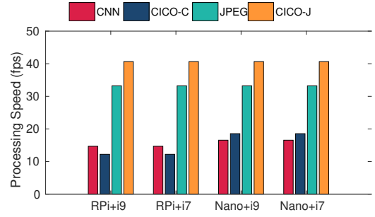
Figure 18: End-to-end image processing rate over WiFi (DET).
