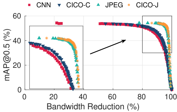
Figure 10: Accuracy-bandwidth trade-offs (DET).
