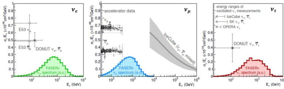
Figure 34. Existing constraints on neutrino CC interaction cross sections, and the expected energy spectra of neutrinos interacting in FASERν. Reproduced from [385]. CC BY 4.0.
