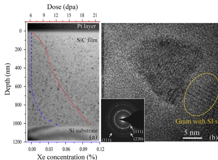
Figure 10. (a) TEM images of amorphous SiC film irradiated with 5 MeV Xe ions at 700 K to a fluence of 1.15 \times 10^{16} ions/cm 2 , with overlaid ion implantation and dose profiles; (b) HR-TEM images and inset SAED showing cubic-structured crystallite formation. Reproduced with permission from ref. [54].
