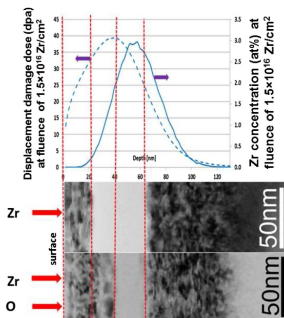
Figure 9. Cross-sectional TEM images of \alpha - \text{Al}_2\text{O}_3 (a) irradiated with \text{Zr}^+ ions to 1.5 \times 10^{16} ions/cm 2 and subsequently with (b) \text{O}^+ ions to 2.3 \times 10^{16} ions/cm 2 , demonstrating the extent of recrystallization of the buried amorphous layer. Overlaid SRIM damage and ion range profiles show a clear relationship between the observed phase structures and the irradiation damage and \text{Zr}^+ ion implantation peaks (red dotted lines). Reproduced with permission from ref. [51].
