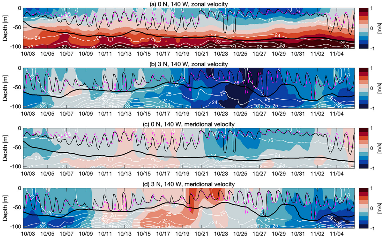
FIG. 9. Time series of zonal and meridional velocity (color), temperature (white contours; °C), mixed layer depth (MLD; dashed magenta), the depth where the bulk Richardson number Ri_b = 0.2 ( H_{Rb} ; thin black), and the base of the low-gradient Richardson number layer Ri_g < 0.35 ( H_{Rig} ; thick black) in the LES at 0° and 3°N along 140°W. All fields are defined from horizontally averaged profiles. The MLD is defined to be the shallowest depth where water is 0.015 \text{ kg m}^{-3} denser than the top 10 m in the instantaneous but horizontally averaged density profile. All time tick marks are at 0000 UTC; local solar time at 0°, 140°W is about 9 h behind UTC, so local solar noon is at about 2100 UTC.
