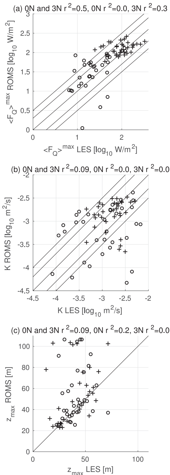
FIG. 19. Comparisons between the LES and ROMS (KPP) at the LES locations (+ at 0° and o at 3°N along 140°W): (a) the maximum turbulent heat flux \langle F_Q \rangle^{\max} , (b) the turbulent diffusivity of heat K at z_{\max} , and (c) the depth z_{\max} at which \langle F_Q \rangle^{\max} occurs. Note, however, that
