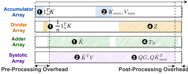
Fig. 7. Illustrating the intra-layer pipeline design that minimizes both the pre- and post-processing overheads for enhancing the overall throughput.
