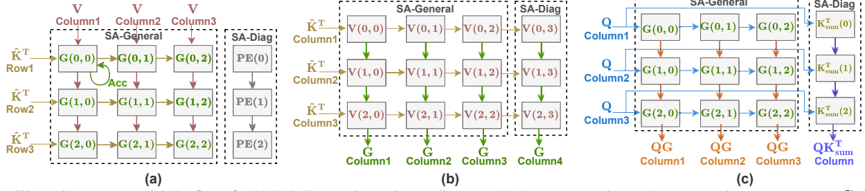
Fig. 9. Illustrating two potential dataflows for ViTALiTY accelerator's systolic array: 1) G -stationary adopts (a) output stationary to compute G = \hat{K}^T V and (c) input stationary to process both QG and QK^T_{sum} for keeping G stationary within the PEs, and 2) down-forward accumulation dataflow that adopts input stationary to handle all the multiplications (see (b) and (c)).
