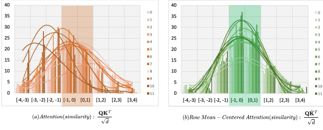
Fig. 3. Distribution of attentions (inputs to softmax) across various layers 0-11: (a) the vanilla attention distribution shifts left, and (b) row-wise mean-centering of attentions centers the distribution towards [-1, 1] . Here we use the DeiT-Tiny [38] model on the ImageNet dataset as an example.
