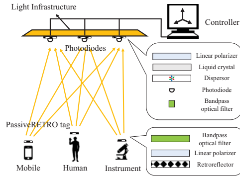
Fig. 2: PassiveRETRO system diagram
