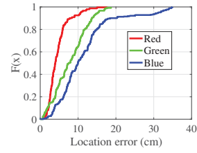
Fig. 17: CDF of 3D location error for multiple devices
