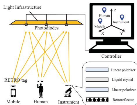
Fig. 1: The architecture of RETRO system
