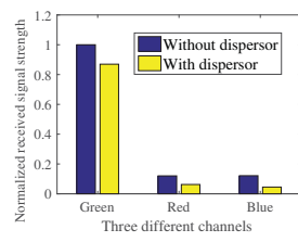
Fig. 11: RSS of green channel with and without dispensor
