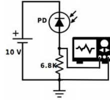
Fig. 9: Light intensity measurement circuit
