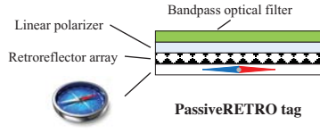
Fig. 4: Structure of PassiveRETRO tag
