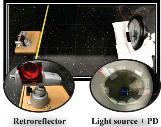
Fig. 8: Testbed of the PassiveRETRO system
