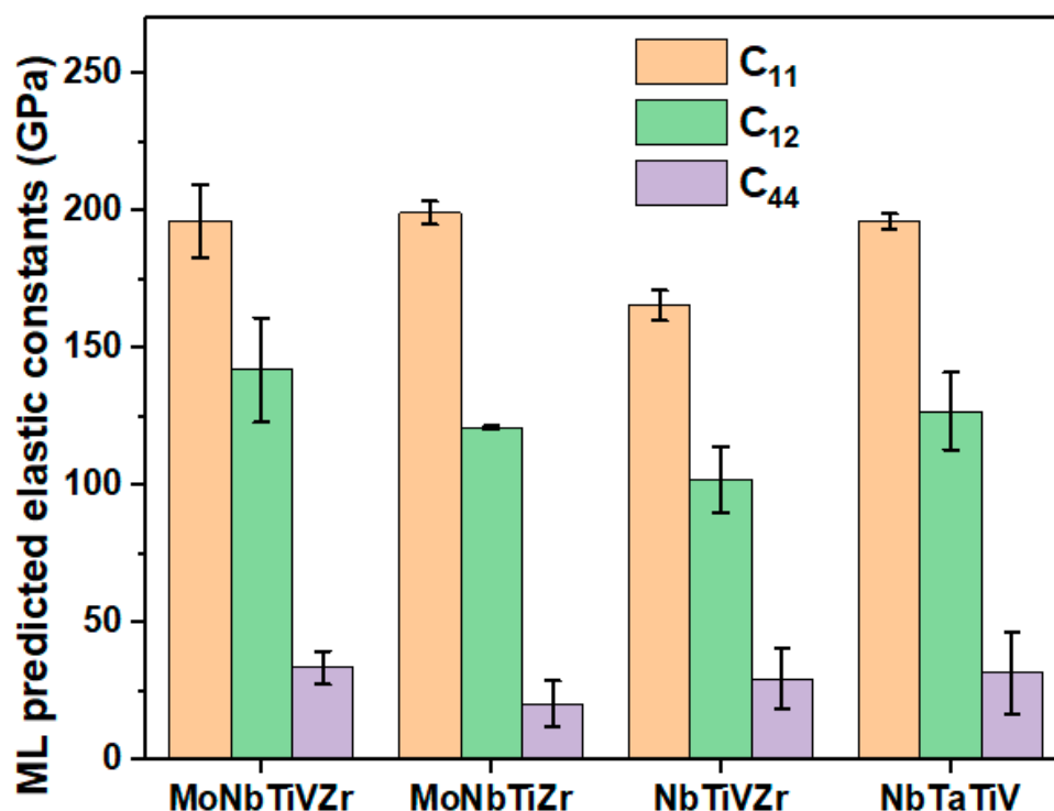
Figure 6. Elastic constants ( C_{11} , C_{12} , and C_{44} are in unit GPa) for MoNbTiVZr, MoNbTiZr, NbTiVZr, and NbTaTiV refractory alloys predicted by the GBR model. The error bar shows how far the elastic constant value has deviated from its original value.
