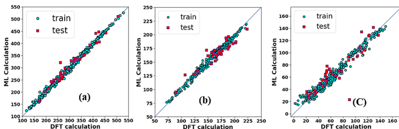
Figure 5. ML-predicted elastic constants of (a) C 11 , (b) C 12 , and (c) C 44 , as a function of DFT-predicted elastic constant during training and testing datasets.
