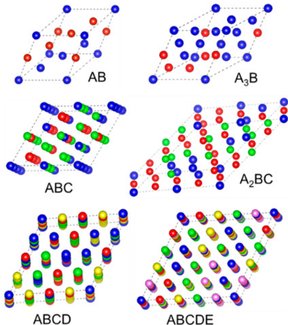
Figure 1. Different SQS models used to calculate the elastic constants of RCCAs.
