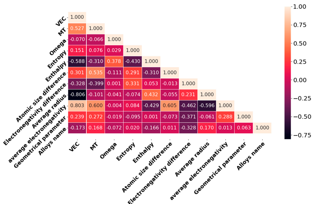
Figure 3. Lower triangular heatmap diagram of 11 descriptors of the initial datasets.
