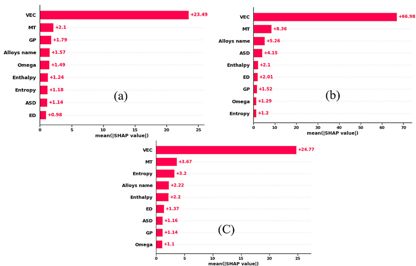
Figure 7. (a–c) Shows the SHAP value for C_{11} , C_{12} , and C_{44} , respectively.
