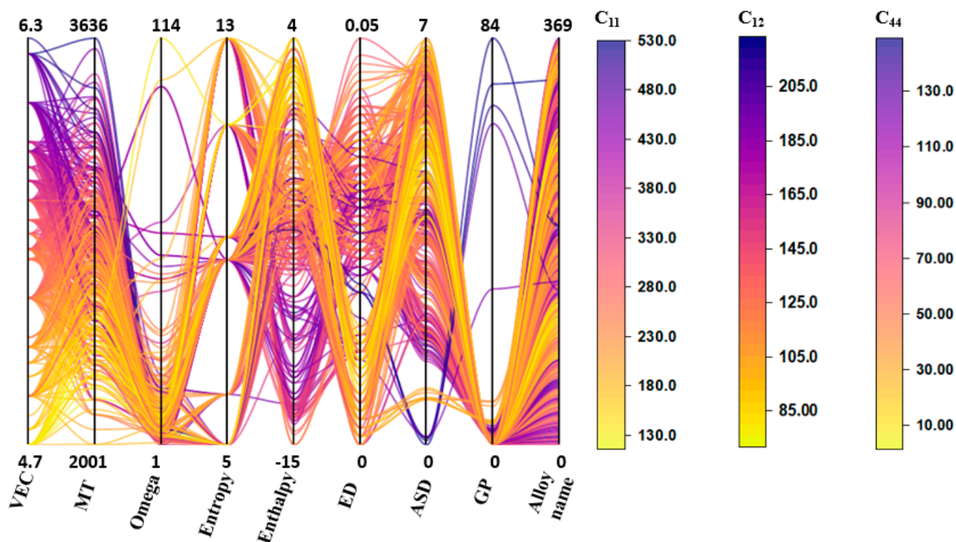
Figure 8. Parallel coordinate plots of elastic constants ( C_{11} , C_{12} , and C_{44} are in GPa) from the datasets.
