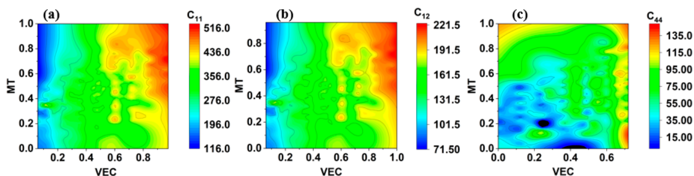
Figure 9. (a–c) Represents the contour plot of elastic constants C_{11} , C_{12} , and C_{44} , respectively.
