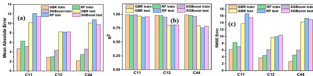
Figure 4. (a–c) Represents the MAE, R^2 , and RMSE of different ML models used, respectively.
