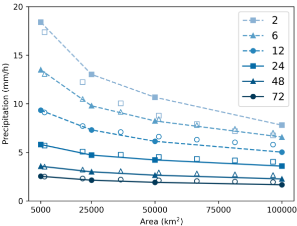
700 Figure C1. Comparison of DAD curves estimated from vine copulas (solid markers) and ARFs from Kao et al., 2020 (empty makers) for Ohio River Basin with 10-year ARI and 2-72 hours durations.
