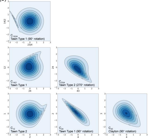
295 Figure 3. (a) A vine copula tree structure for atmospheric water balance components ( d = 4 ), where 1, 2, 3, and 4 represent water balance components. Note that the permutation is not unique and depends on model fitting; (b) Normalized bivariate copula contour plots of all pair copulas specified in the copula tree structure in (a). The contour colors represent the copula densities.
