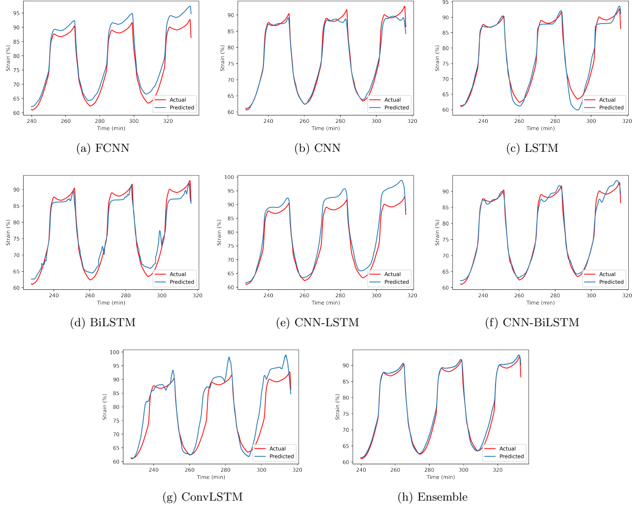
Figure 8: Prediction performance for dataset 2 by the following DL models: (a) FCNN, (b) CNN, (c) LSTM, (d) BiLSTM, (e) CNN-LSTM, (f) CNN-BiLSTM, (g) ConvLSTM, and (h) Ensemble.
