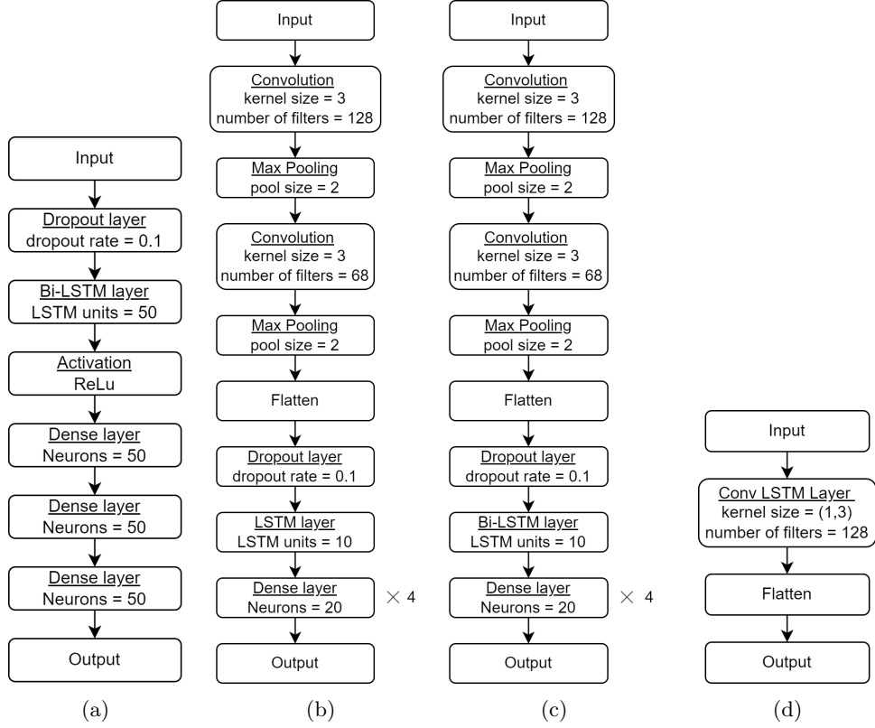
Figure 6: Visual representation of hybrid neural network models where (a) shows the BiLSTM model, (b) shows the CNN-LSTM model, (c) shows the CNN-BiLSTM model, and (d) shows the ConvLSTM model.
