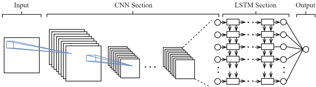
Figure 14: General CNN-LSTM.
