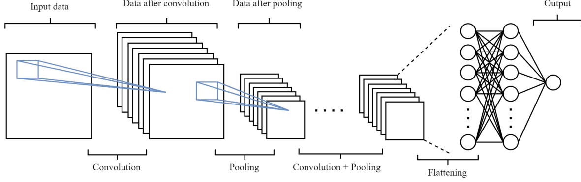
Figure 11: General CNN.
