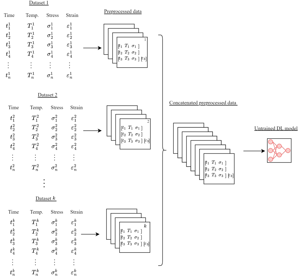
Figure 1: Training process of DL model.
