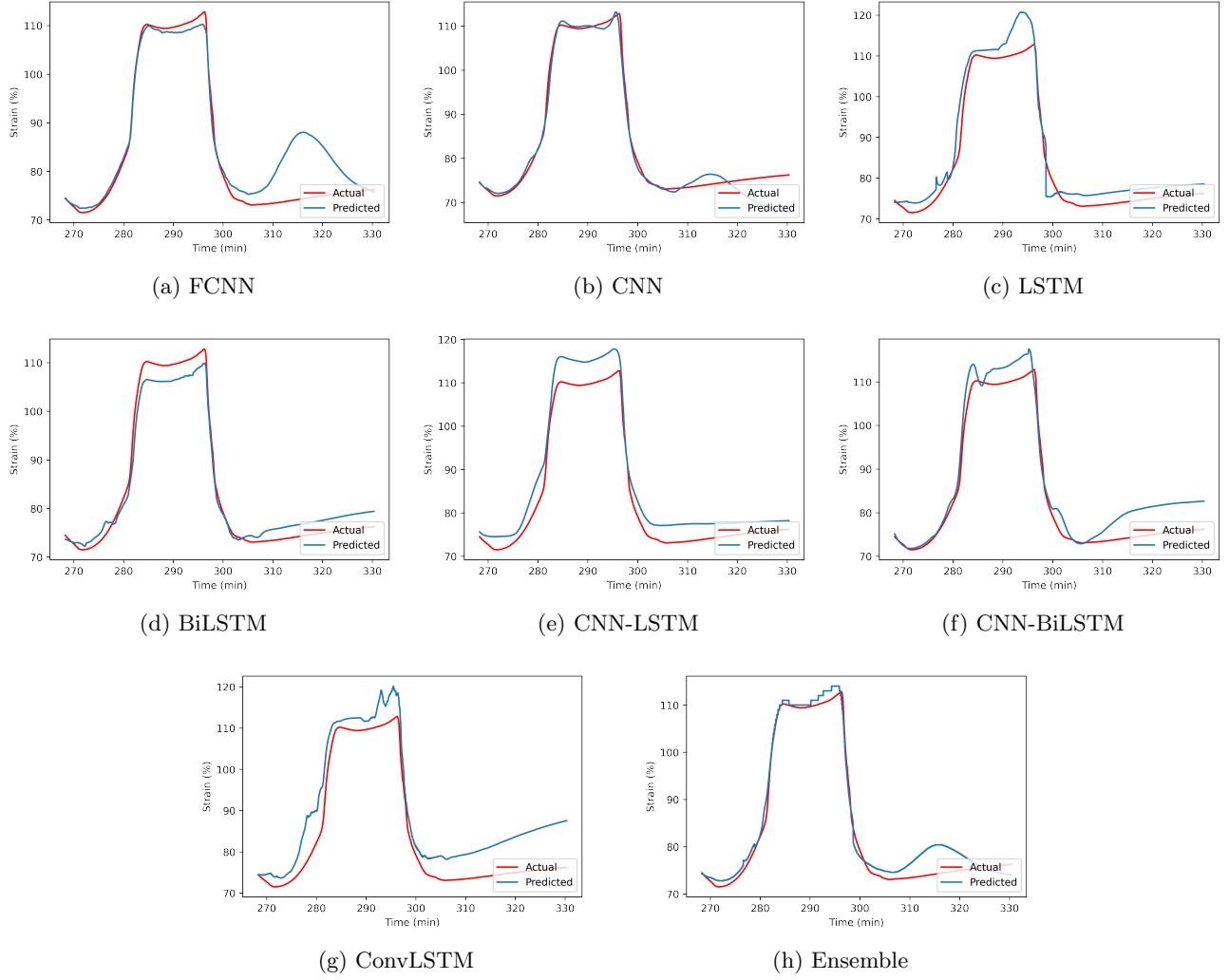
Figure 7: Prediction performance for dataset 1 by the following DL models: (a) FCNN, (b) CNN, (c) LSTM, (d) BiLSTM, (e) CNN-LSTM, (f) CNN-BiLSTM, (g) ConvLSTM, and (h) Ensemble.
