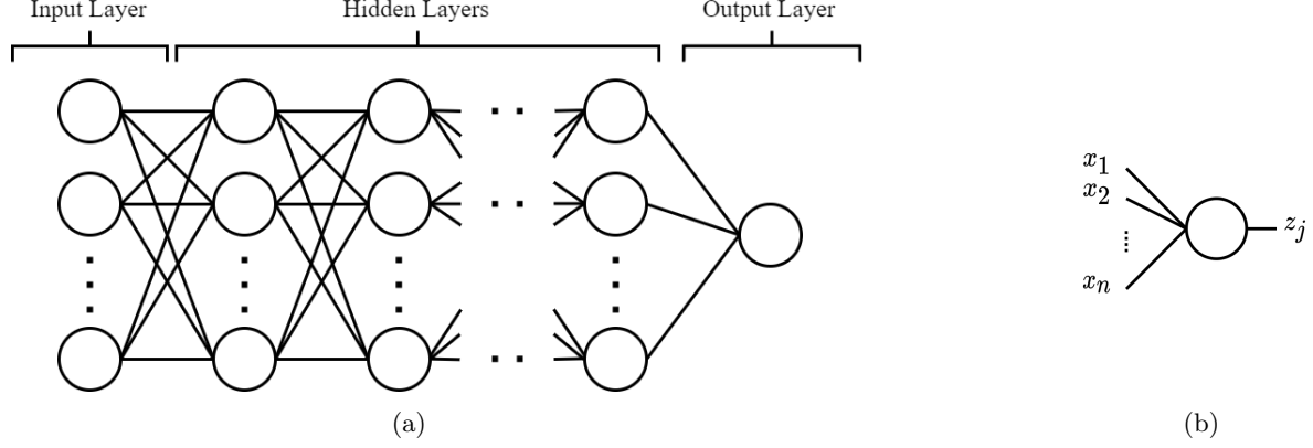
Figure 10: Visual representation of a general FCNN where (a) shows the complete FCNN model and (b) shows a section of the FCNN model displaying a single neuron.
