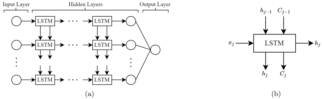
Figure 12: (a) General LSTM process. (b) Detailed representation of how data is transferred in a single LSTM cell.
