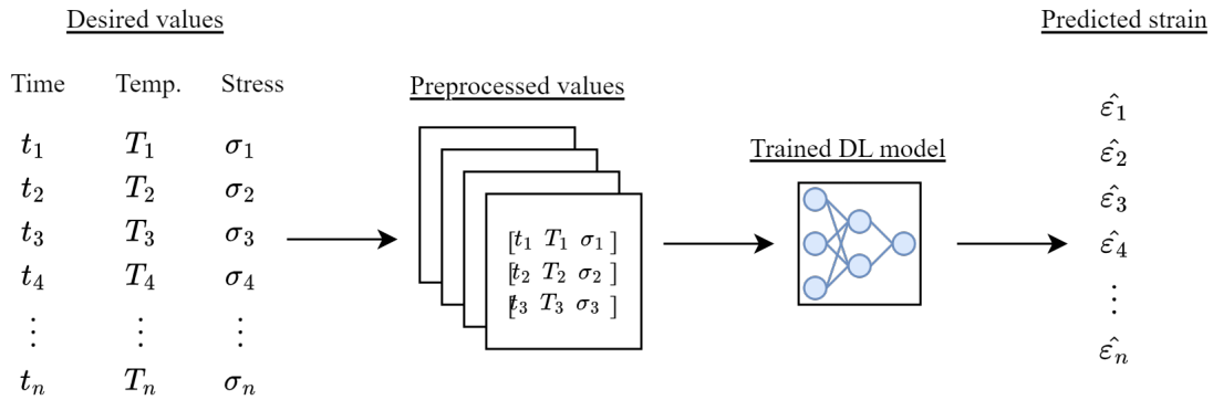
Figure 2: Prediction process to find the change in strain.
