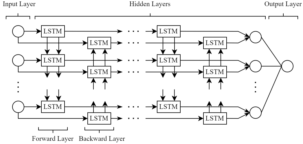
Figure 13: General BiLSTM.
