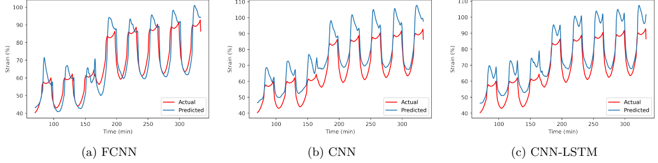
Figure 9: Prediction performance for dataset 2 by the following DL models: (a) FCNN, (b) CNN, and (c) CNN-LSTM.
