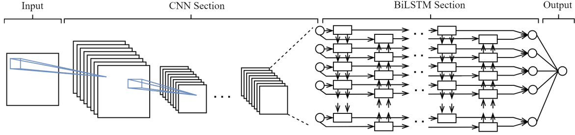
Figure 15: general CNN-BiLSTM.
