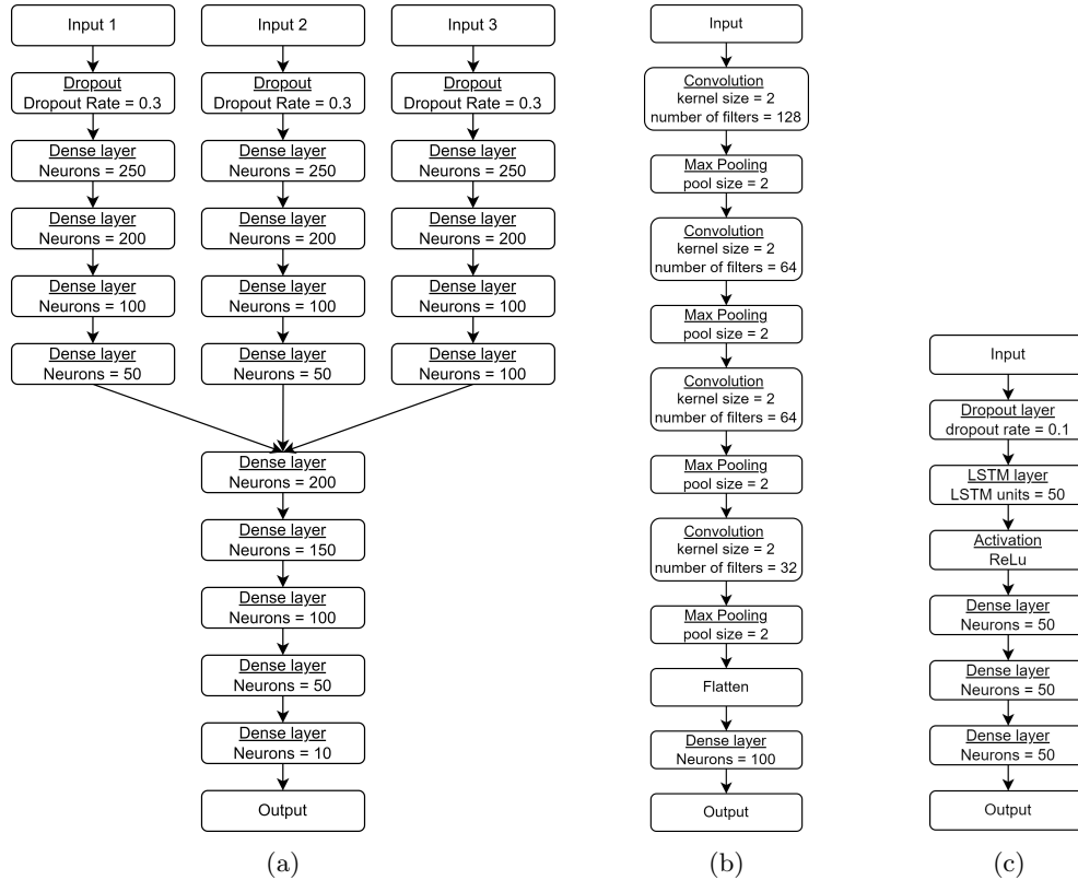
Figure 5: Visual representation of core neural network models where (a) shows the FCNN model, (b) shows the CNN model, and (c) shows the LSTM model.
