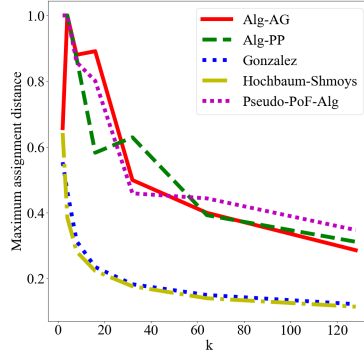
Figure 8: Maximum assignment distance for all algorithms
