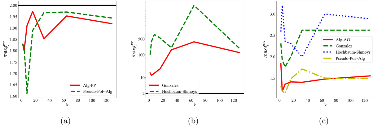
Figure 3: Satisfaction of fairness constraints
