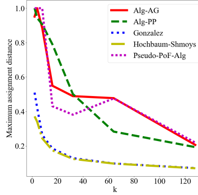
Figure 2: Maximum assignment distance for all algorithms
