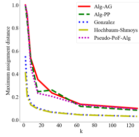
Figure 5: Maximum assignment distance for all algorithms
