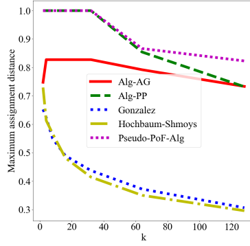
Figure 11: Maximum assignment distance for all algorithms
