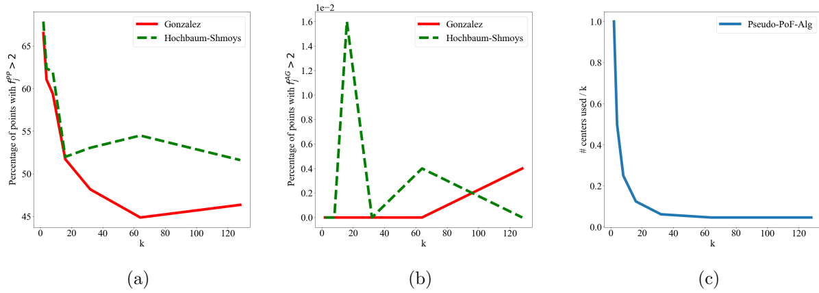
Figure 13: Amount of constraint violation
