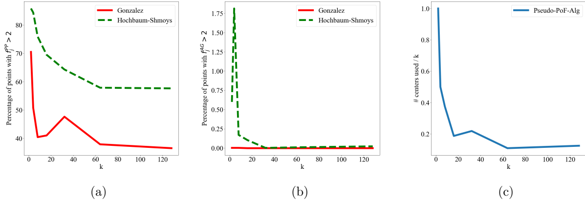
Figure 10: Amount of constraint violation
