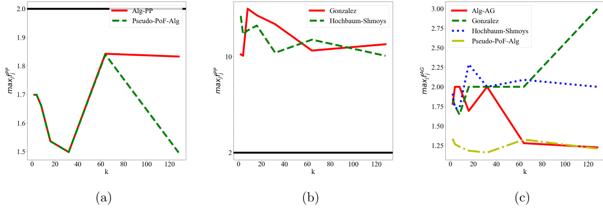
Figure 12: Satisfaction of fairness constraints
