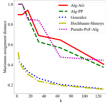
Figure 14: Maximum assignment distance for all algorithms
