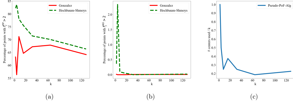
Figure 4: Amount of constraint violation
