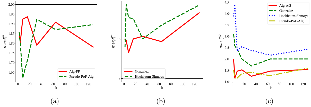
Figure 9: Satisfaction of fairness constraints
