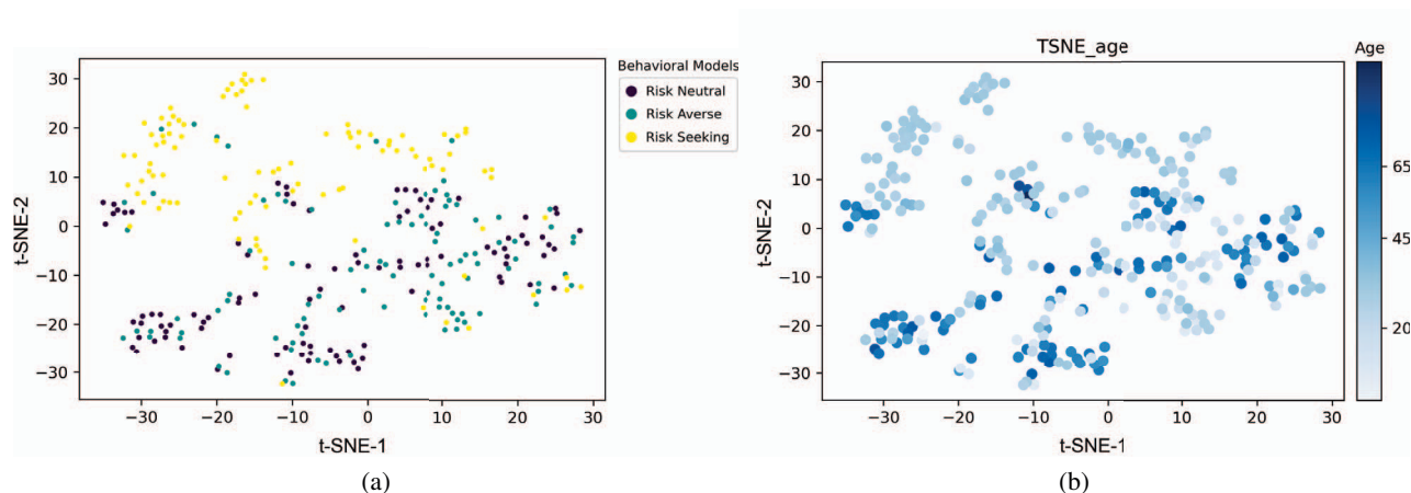
Figure 1: Three behavioral models formulated based on the age and household size of the agent (Model I). Weight vectors of the reward functions after dimensionality reduction from 440 to two by the t-SNE algorithm (a) illustrate the behavioral model assigned to the agents by color labels, The appeared clustering patterns suggest that even though agents are assigned with three equality different behavioral models, the emerging behavior of risk-neutral and risk-averse agents are more similar compared to emerging behaviors of risk-seeking agents; (b) This shows how correlation of age with risk seeking model partially contributes to the differentiation of emerging behaviors.
