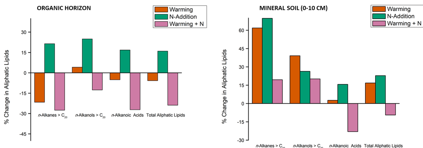
Figure 1. Concentration of aliphatic lipids reported as percent change relative to control as measured in organic and mineral (0–10 cm) soil samples. n -Alkanes and n -alkanols with chain length <C 20 were not detected (Tables S1 and S2).
