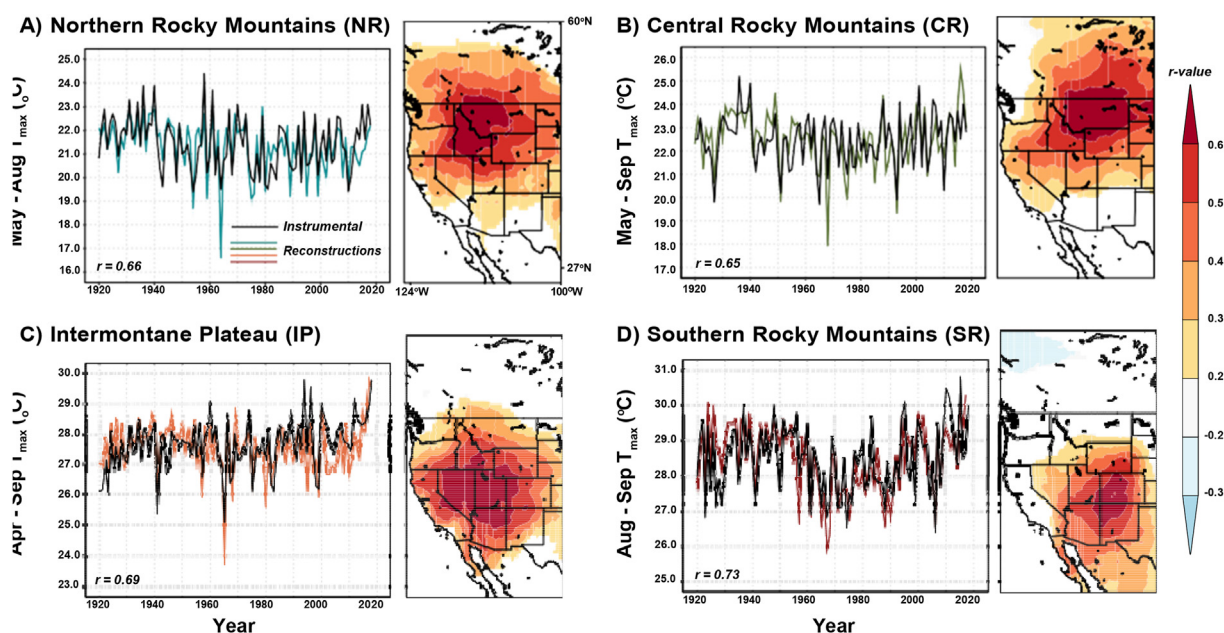
Fig. 3. Temporal and spatial relationships between 4 western US regional maximum temperature ( T_{\max} ) reconstructions and instrumental data. The temporal relationship (Pearson's r , p < 0.05 ) between the regional reconstructions (colored lines, line shading represents standard error) and the CRU TS 4.04 T_{\max} data (black line) (Harris et al., 2014) over the period spanning 1920–2018. We also include the extent of the spatial distribution of correlations between the predictor and predictand temperature data for each regional model over the period 1920–2018 (Pearson's r , significant at p < 0.05 level).
