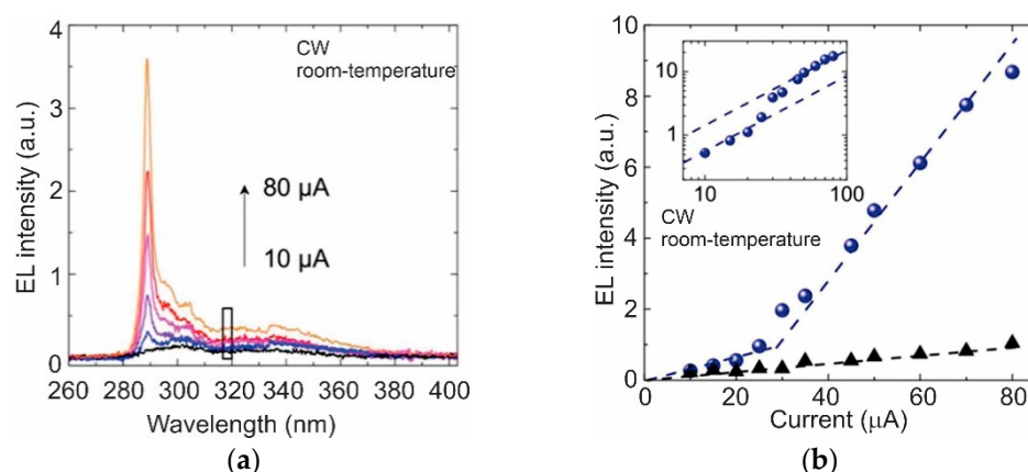
Figure 13. UV-C laser characteristics at RT, (a) EL emission spectra measured under different current densities, and (b) integrated EL intensity as a function of the injection current. Figures are reproduced with permission from reference [27]. Copyright (2015) AIP Publishing LLC.
