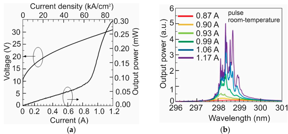
Figure 9. (a) L-I-V characteristics for the UV-B lasers, and (b) emission spectra of the laser at different current bias. Figures are reproduced with permission from reference [31]. Copyright (2020) The Japan Society of Applied Physics.
