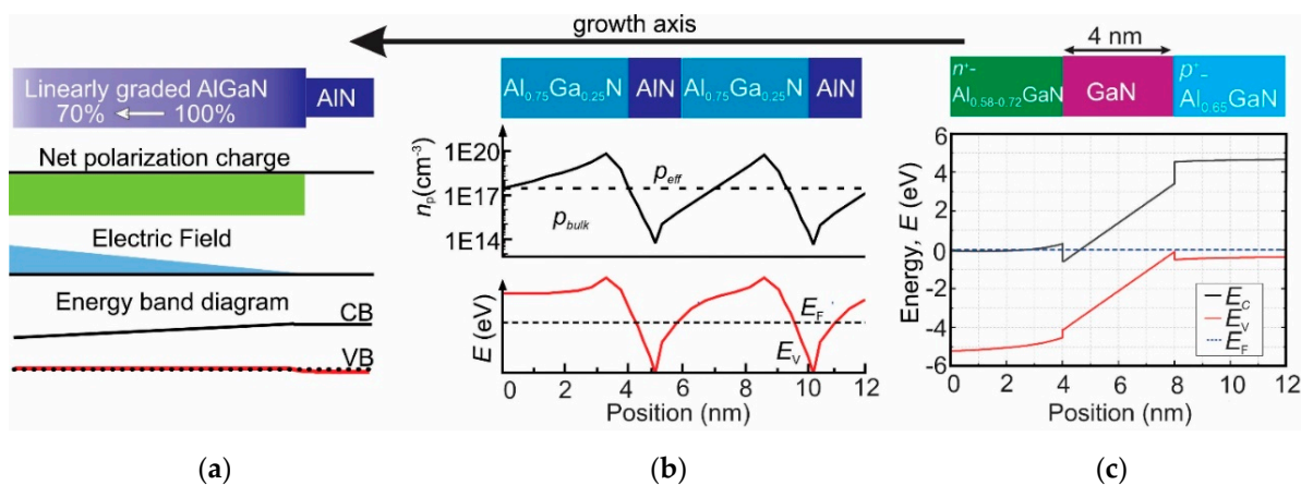
Figure 6. Schematic representation of the p -doping process; (a) schematic representation of distributed polarization doping (DPD) process for an AlGaIn layer graded from x = 0.7 to 1, (b) a schematic representation of short-period superlattice (SPSL) with \text{Al}_{0.75}\text{Ga}_{0.25}\text{N}/\text{AlN} alternate layers doped with 3.5 \times 10^{19} \text{ cm}^{-3} Mg generated. The dotted line represents the hole concentration for bulk \text{Al}_{0.75}\text{Ga}_{0.25}\text{N} with equal doping, and (c) band diagram of a p -AlGaIn/ i -InGaIn/ n -AlGaIn TJ.
