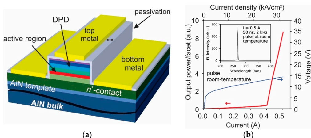
Figure 7. (a) Schematic cross-section of fully-processed UV-C laser and (b) its L-I-V characteristics. (b) is reproduced with permission from reference [30]. Copyright (2019) The Japan Society of Applied Physics.
