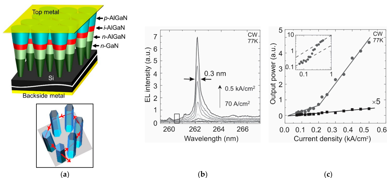
Figure 12. (a) Three-dimensional schematic representation of the fully-processed random lasers. Inset shows the mechanism for random laser emission, (b) electroluminescence (EL) emission spectra measured under different current densities, and (c) integrated EL intensity as a function of the injection current for the NW laser. Figures are reproduced with permission from Reference [28]. Copyright (2015) AIP Publishing LLC.
