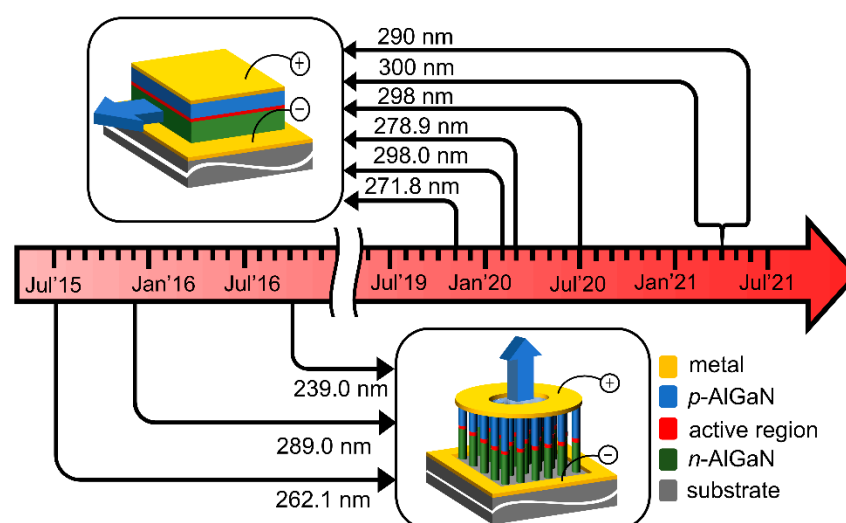
Figure 2. All key demonstrations [27–36] for electrically-pumped AlGaIn lasers covering ultraviolet (UV)-B and -C wavelengths since 2015.
