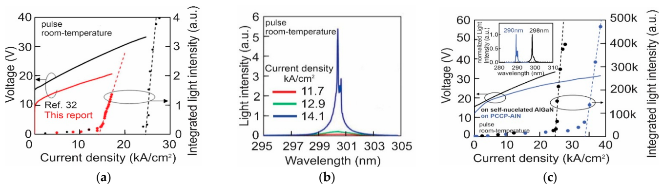
Figure 11. L-J-V characteristics of the UV-B laser with p -electrode width of 10 \mu\text{m} plotted along with the UV-B laser reported in reference [32], (b) emission spectra of the laser with p -electrode width of 15 \mu\text{m} at different current bias, (c) L-J-V characteristics of the UV-B laser grown on different AlGaN template. The lasing spectra are shown in the inset. (a,b) are reproduced with permission from reference [35]. (c) is reproduced with permission from Reference [36]. Copyright (2021) The Japan Society of Applied Physics.
