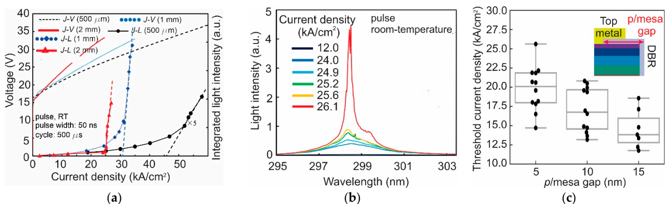
Figure 10. (a) L-J-V characteristics, (b) electrical current density dependent emission spectra of the UV-B lasers, and (c) threshold current density with respect to different p/mesa gap widths. (a,b) are reproduced with permission from reference [32]. Copyright (2020) The Japan Society of Applied Physics (c) is reproduced with permission from Reference [34]. Copyright (2021) The Japan Society of Applied Physics.
