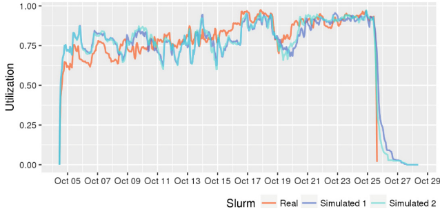
Fig. 12. Comparison of resource utilization between historical Slurm run and two simulated runs.
