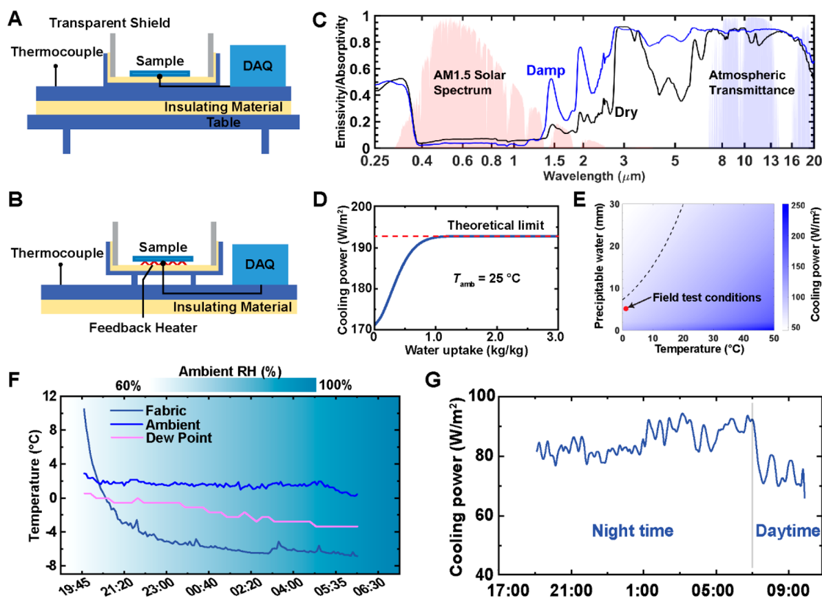
Figure 3. Optical and thermal characterization of the cellulose-based fabric with field validation. (A) Schematic of the temperature measurement setup. (B) Cooling power experimental setup. The sample was maintained at the same temperature as the ambient by a feedback heater. The power output of the feedback heater is regarded as the cooling power. (C) Emissivity in the ultraviolet, visible, and infrared range of the fabric under dry and damp conditions. (D) Theoretical cooling power as a function of water uptake of the fabric sample. (E) Theoretical cooling power as a function of precipitable water and ambient temperature. The dashed line traces PW of 100% RH at different ambient temperatures. (F) Profiles of the sample surface temperatures and ambient temperature on Nov 11, 2020. The RH is represented by the colored background. The sample's temperature dropped rapidly at the beginning of the field test because of the high initial temperature. (G) Profile of the cooling power measured between 19:00 and 9:30 on Jan 20, 2021. The ambient conditions of the field test are also indicated in panel E.
