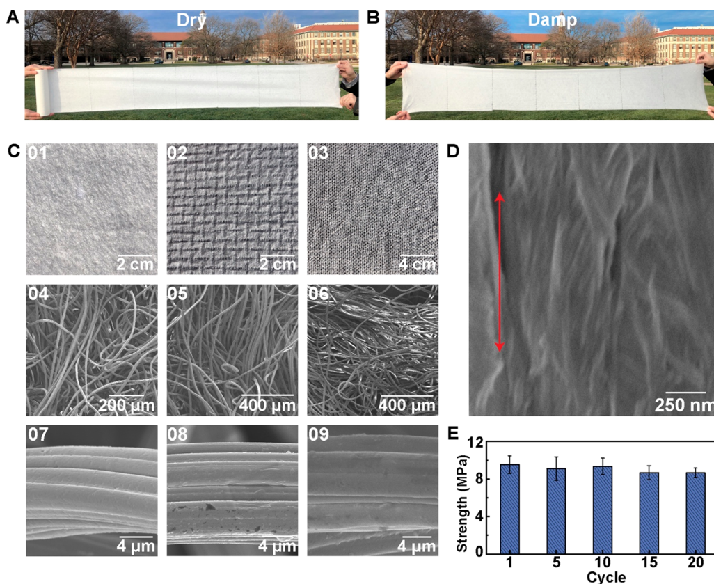
Figure 2. Macro-/microstructures and mechanical properties of cellulose fabric. Photographs of large-scale cellulose fabric under (A) dry and (B) damp conditions with a width of 25 cm. (C) (01–03) Photographs and (04–06) SEMs of different fabric samples composed of entangled cellulose fiber bundles and (07–09) magnified views of fibers within bundles. The images in the same column are from the same sample. (D) SEM image of partially aligned nanofibers. The arrow indicates the nanofiber alignment direction. (E) Mechanical strength over 1, 5, 10, 15, and 20 adsorption–extraction cycles of the fabric sample.
