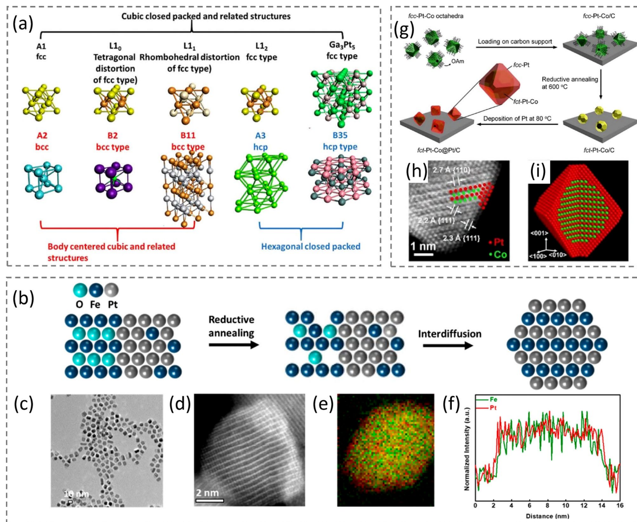
Fig. 8 a Illustration of some simple alloy structures and their corresponding intermetallic structures. b Schematic of structural conversion from dumbbell-like Fe 3 O 4 -PtFe NPs to L1 0 -PtFe via reductive annealing. c–f TEM image of dumbbell-like Fe 3 O 4 -PtFe alloy nanoparticles. d–f HAADF-STEM image, elemental map, and line-scanning profile of the converted L1 0 -PtFe nanoparticle, respectively. Reproduced with permission from Ref. [11] and modified. Copyright 2009 American Chemical Society. g Schematic illustration of the three major steps involved in a typical synthesis of fcc -Pt-Co@Pt/C catalyst. h Atomic-resolution STEM image of the Pt-Co@Pt octahedral nanocrystal along the [110] direction. i Schematic of this nanocrystal featuring an intermetallic core, a Pt shell of about three atomic layers thick, and (111) facets. The red- and green-colored atoms correspond to Pt and Co, respectively. Reproduced with permission from Ref. [114]. Copyright 2021 American Chemical Society
