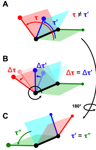
Figure 2: A: The torsion \tau around a bond depends on a choice of neighbors. B: The change \Delta\tau caused by a relative rotation is the same for all choices. C: The sign of \Delta\tau is unambiguous because given the same neighbors, \tau does not depend on bond direction.
