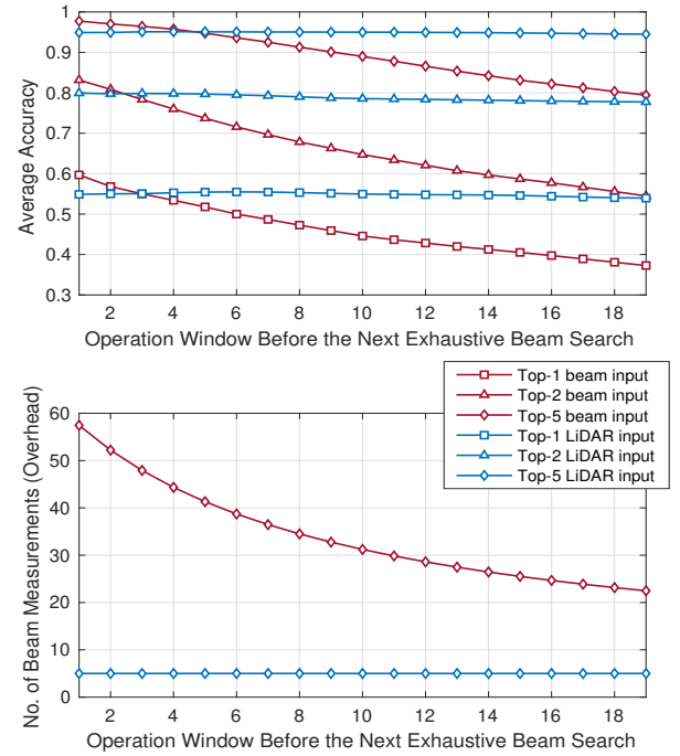
Fig. 3. This figure shows the accuracy performance of the two future beam prediction approaches with different operation windows. The LiDAR-aided solution can keep track of the beam with lower training overhead.
