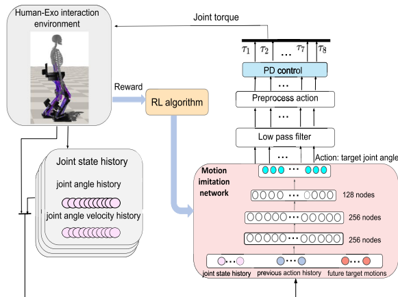
Fig. 3 RL-based motion imitation control of the LLRE (the LLRE control loop in Fig. 2). The inputs of the motion imitation network consist of the joint state history, the action history and the future target motions. This learning network outputs joint target positions, which are processed by a low-pass filter and then translated into torque-level commands by PD control
