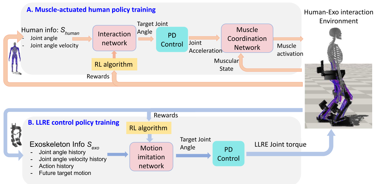
Fig. 2 Overview of the modular, decoupled RL-based walking control framework of the LLRE with human-in-the-loop. The framework is separated into two parts: A muscle-actuated human policy training. B LLRE control policy training, which integrates three deep neural networks (marked with pink blocks): an RL-based interaction network for human control to manage human-exoskeleton interface forces; a supervised muscle coordination network for whole body muscle control; a RL-based motion imitation network for the control of the LLRE. The muscle-actuated human control loop A is designed to learn human muscle coordination giving the health status of the human and predicted exoskeleton assistance. The LLRE control loop B is designed to imitate a target walking motion while maintaining strong robustness and balance under the human-exoskeleton interaction. These three networks can be jointly trained in the simulation while they interact with each other to achieve maximum rewards during RL
