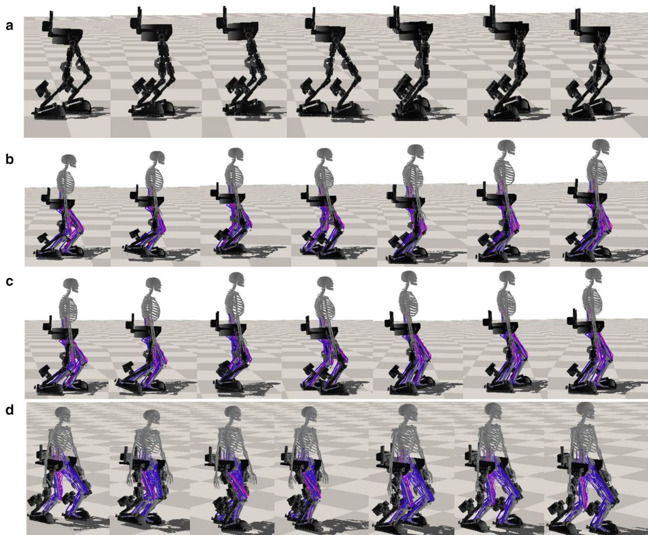
Fig. 4 Snapshots of the walking control of the LLRE. The learned controller trained from the decoupled RL-based control framework enables the LLRE to perform walking assistance under varying human-exoskeleton interactions from human subjects with various neuromuscular disorders. a Autonomous walking control without human involved. b robust walking control with a fully healthy, muscle-actuated human. c robust walking assistance with a human with muscle weakness. d robust walking assistance with a human with left hemiparesis. The color of the muscle indicates its activation, with purple being the highest and blue being the lowest
