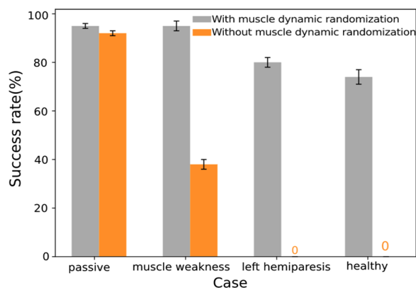
Fig. 10 Ablation study. It shows the comparison results of success rates for different human conditions with/without muscle strength randomization training. The success rate is evaluated over 100 trials for each condition. The success rates in all human conditions are significantly higher than that trained without muscle strength randomization
