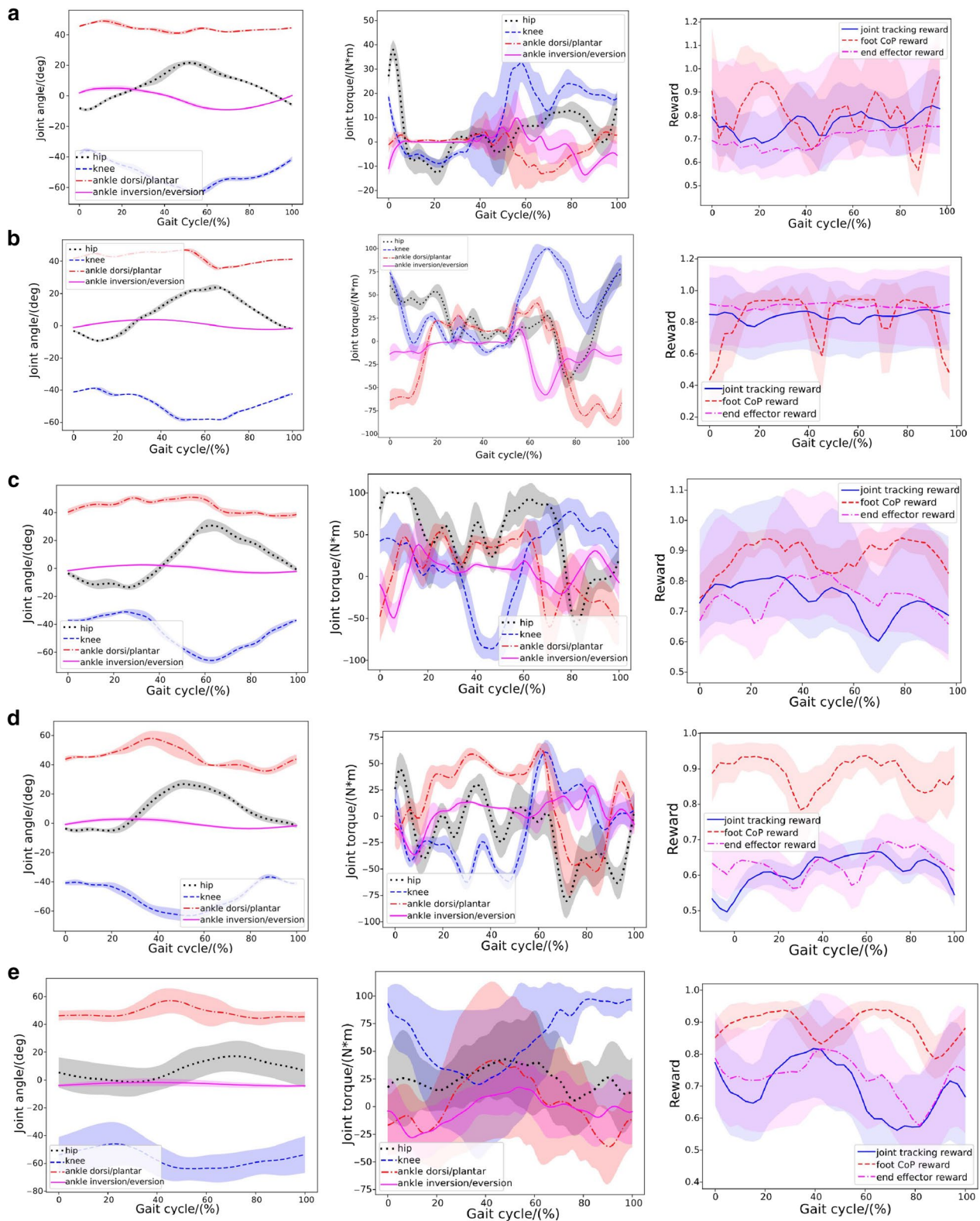
Fig. 5 Statistical analysis results during 40 walking cycles without human or with human subjects under different neuromuscular conditions (curve: mean; shade: STD). From left to right are exoskeleton joint angles, joint torques, and rewards, including the joint position tracking and end-effector reward in Eq. 10 and the CoP reward in Eq. 12. a without a human; b with a passive human; c with a healthy human; d with a human with muscle weakness; e with a human under the left hemiparesis condition
