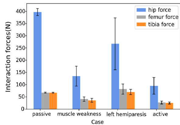
Fig. 11 Human-exoskeleton interaction (strap) forces under different cases during 40 walking cycles
