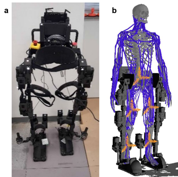
Fig. 1 The integrated human and exoskeleton model. a The physical prototype of the LLRE. b The integrated musculoskeletal and exoskeleton model. The yellow coordination frames show the bushing frames coincidentally fixed on the LLRE and the human
