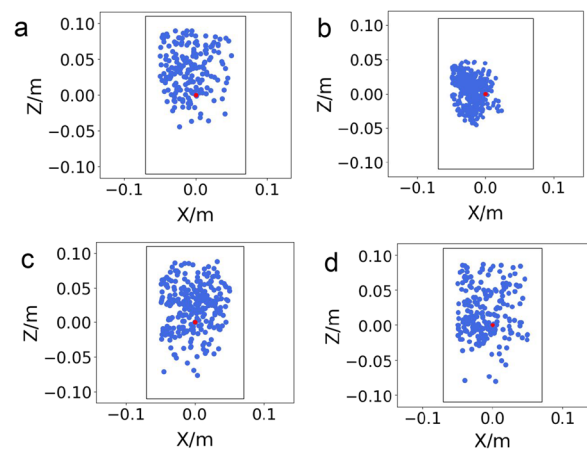
Fig. 9 CoP-based stability analysis. It shows the CoP locations under different human conditions during 100 walking gait cycles. a Fully passive; b healthy; c muscle weakness; and d hemiparesis. We can clearly see that all CoP positions stay inside the stable region during the walking motion
