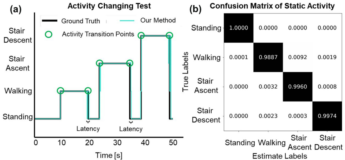
FIGURE 6. The classification results of the activity changing test. (a) Activity detection results. The misclassified timestamps are mainly distributed around the activity transition point as a result of the transition latency. The latency is the time difference between the proposed point where the algorithm detected the transition and the ground truth. The average latency across activities was 236 \pm 177 ms. (b) The confusion matrix for activity detection results shows that for standing the activity classifier is perfect (100%). Moreover, the activity classifier can accurately classify walking (98.87%), stair ascending (99.60%), and stair descending (99.74%), resulting in an average of 99.55% classifier accuracy.
