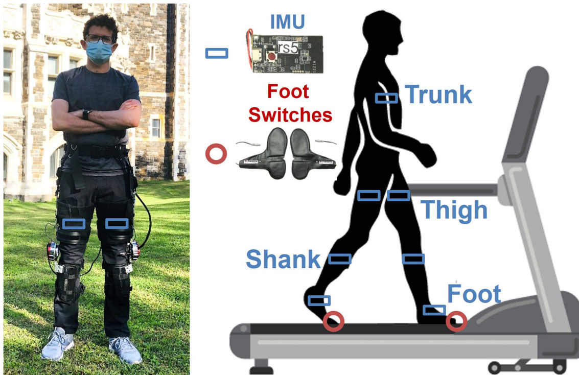
FIGURE 1. Sensing configuration for activity classification, gait phase estimation, and prediction, which can be used for both gait monitoring and robot control. As in the training procedure, the footswitches were used to provide the ground truth of gait phase labeling.
