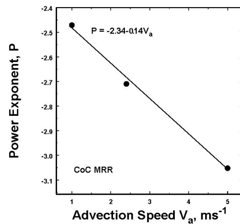
Figure 10. A plot illustrating the effect of increasing advection speed on the slope of a power fit to the radial spectral power function for the CoC data illustrating the importance of using an estimate of an optimal advection speed rather than an arbitrary assumption as was made in [26].
