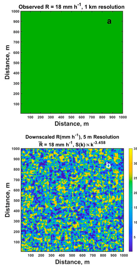
Figure A1. (a) Illustrates the input uniform value as seen, for example, by a radar with a 1 km beam width or as output from a numerical model with a 1 km grid spacing and (b) one realization of the resulting downscaling to 5 m resolution using the indicated radial power spectrum as discussed further in the text.
