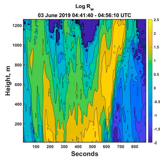
Figure 1. Time–height profile of the logarithm of the rainfall rate as derived in [6] for the so-called early period of 3 June 2019 data.
