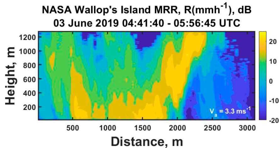
Figure 4. Spatially scaled rainfall rate data in both the vertical and horizontal directions where the distance is the translation distance from the observation location implied by the frozen turbulence advection speed in Figure 3.
