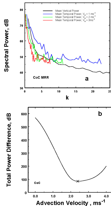
Figure 8. (a,b) are as in Figure 7 except for the CoC data. This time, the optimum V_a = 2.4 \text{ ms}^{-1} .
