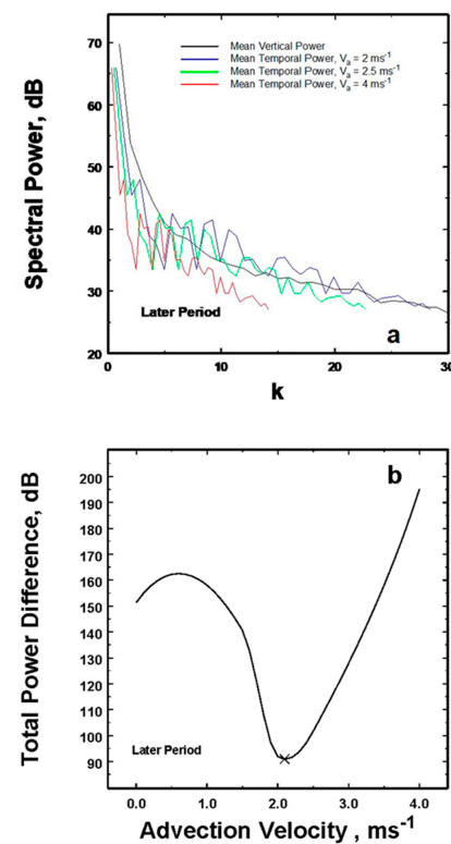
Figure 7. (a,b) are as in Figure 6 except for the later period of the 3 June 2019 data. This time, the optimum V_a = 2.1 \text{ ms}^{-1} .
