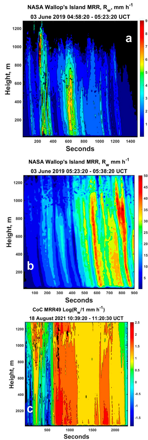
Figure 5. Replot of the rainfall rate time–height profiles for 3 June 2019 for (a) the middle period, (b), the later period, and finally (c) the Charleston College MRR data as deduced in [6] and discussed in the text.
