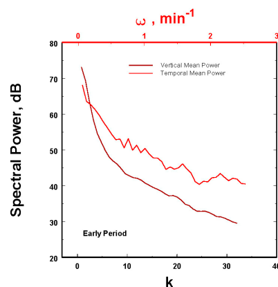
Figure 2. The averaged power spectra as functions of the wavenumber k in space and the frequency \omega in time for the rainfall rates in Figure 1 in both the purely vertical spatial dimension (black) and in the purely temporal domain (red), showing the time and space differences in the spectra.
