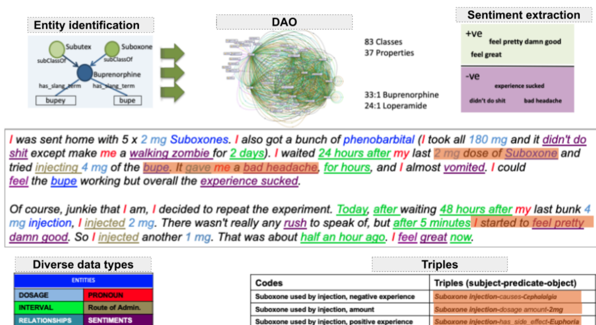
Figure 4. Automatic annotation of texts with the drug abuse ontology (DAO) [80].
