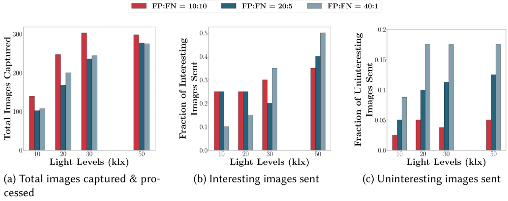
Fig. 9. Figures (a) to (c) show the performance of Camaroptera with different classifiers at different light levels, operating in the Local Inference mode. The different classifiers are represented by their False Positive:False Negative (FP:FN) ratio. Here, the True Positive rate for the environment is set to be 20%. Different classifier FP:FN ratios represent different design points for Camaroptera.
