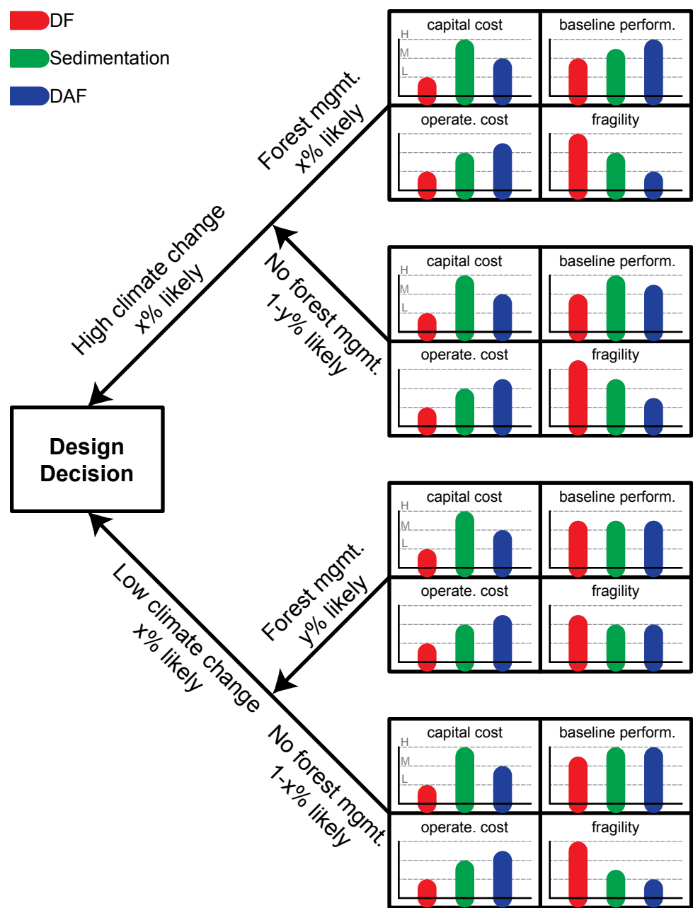
Figure 5. Real options analysis decision tree framework for the comparison of three clarification designs: Direct filtration (DF), gravity sedimentation (e.g., conventional settling), and dissolved air flotation (DAF). Capital and operational costs, and baseline performance taken from Gregory and Edzwald, 2011.
