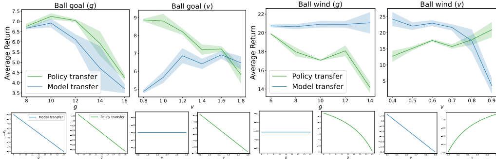
Figure 2: First row: Average return on test tasks v.s. environmental properties ( v and g ). Second row: -K_J v.s. v and g : how -K_J is expected to change based on our theoretical computing results in Table 1. Each plot in the first row is associated with two plots below with corresponding color. The performance of the algorithm is expected to decrease if -K_J decreases.
