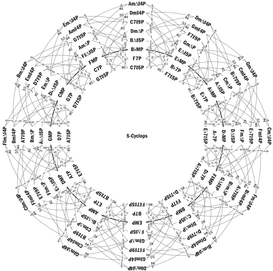
Fig. 4. The 5-Cyclops, with the pentatonic scales considered in Table 5.
