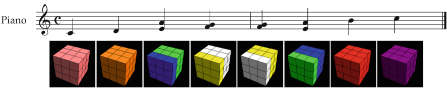
Fig. 8. Musical effect of the rotation of Fig. 7.
