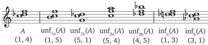
Fig. 1. Examples of unfoldings and infoldings of a chord.
