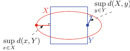
Fig. 5. Calculation of the Hausdorff distance between two metric spaces X (the ellipse) and Y (the square).
