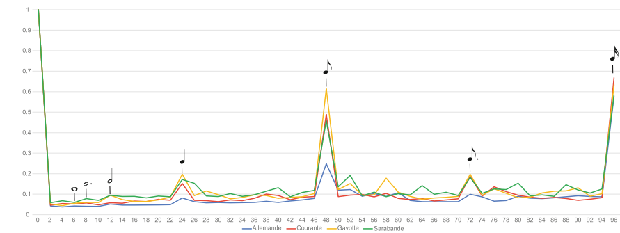
Fig. 2. Average DFT values for each metric type at (\delta, \gamma, \tau) = (6, 3, 1) .
