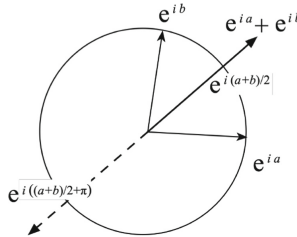
Fig. 1. Sum and phase of two complex numbers with the same length.
