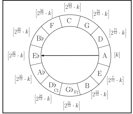
Fig. 1. The circle of fifths
