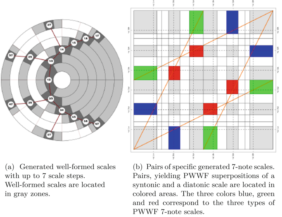
Fig. 2. Types of PWWF 7-note scales and their superpositions.
