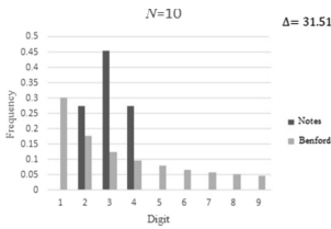
Fig. 2. The first 10 values of the note frequency formula
