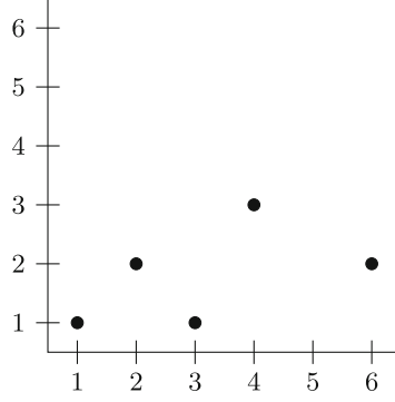
Fig. 1. Example point set
