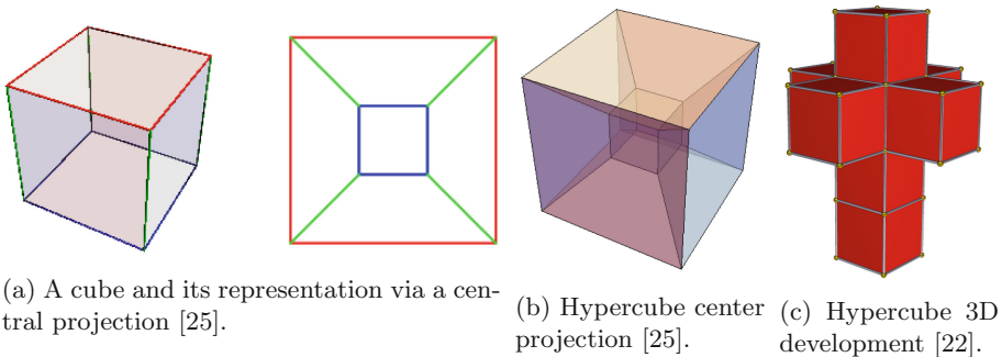
Fig. 3. Some representations of cube and hypercube.
