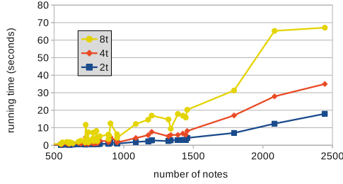
Fig. 3. Efficiency of the algorithm for max_d values 2t , 4t and 8t where t denotes the number of ticks in a beat.
