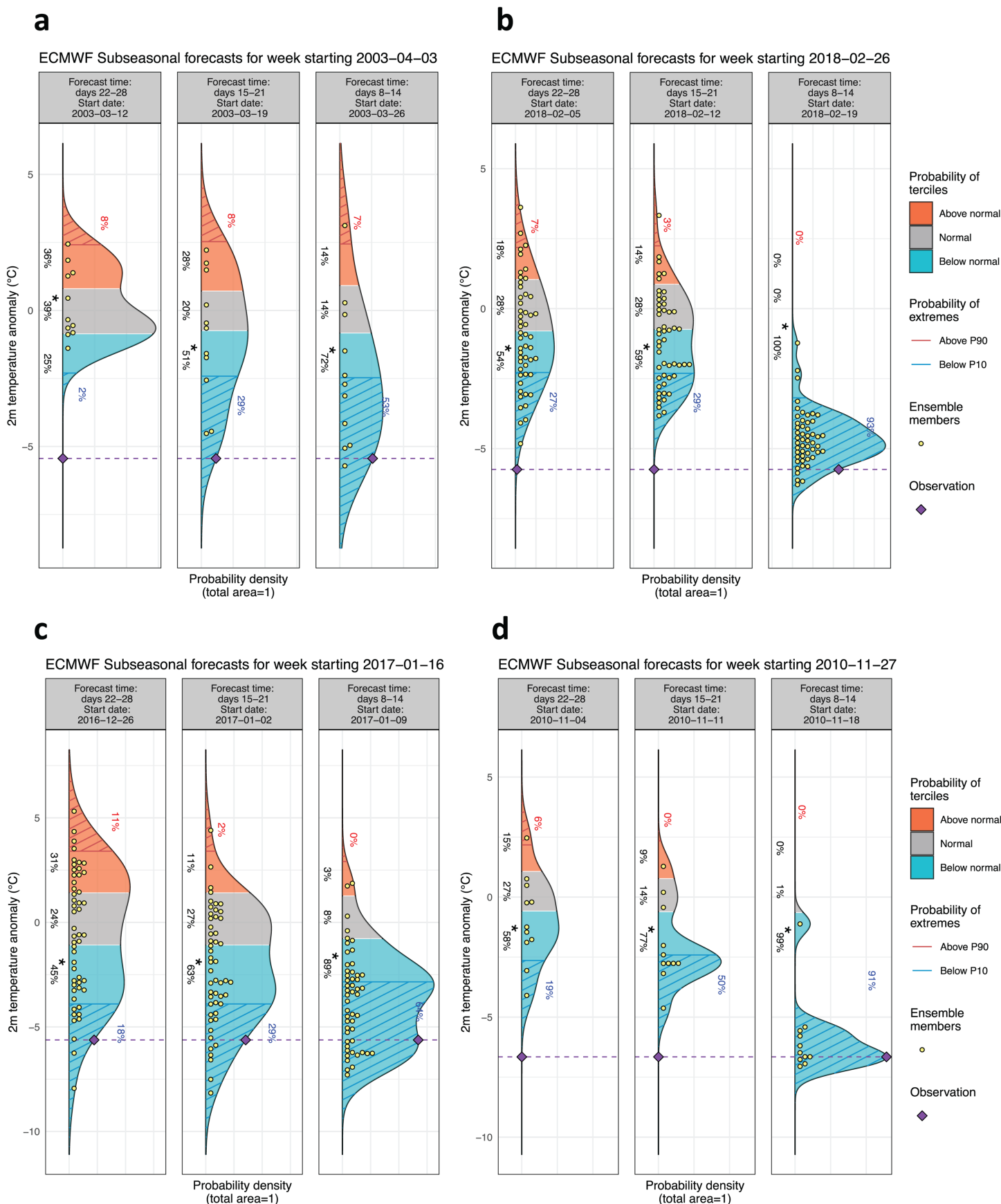
Fig. 4. As in Fig. 2, but for the cold spell case studies: (a) Southeastern European cold spell in 2003, (b) European cold spell in 2018, (c) France cold spell in 2017, and (d) the northern European cold spell in 2010.
