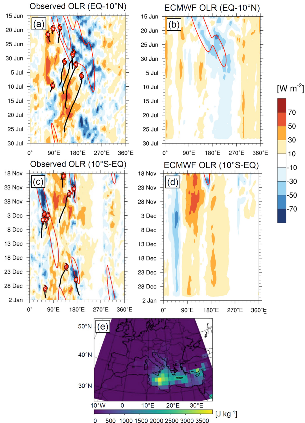
Fig. 8. Cyclones: Outgoing longwave radiation (OLR) anomalies (shaded; \text{W m}^{-2} ) and MJO-filtered OLR anomalies (red contours; every 15 \text{ W m}^{-2} for negative values) from (a),(c) observations averaged over (a) 0^{\circ} – 10^{\circ}\text{N} and (c) 0^{\circ} – 10^{\circ}\text{S} with tropical cyclone tracks (black lines) and names (first letter of the cyclone name in the red circle) and (b),(d) ECMWF ensemble forecasts initialized on 15 Jun 2015 and 18 Nov 2019. MJO filtering is performed using a wavenumber–frequency filter that selects for wavenumbers 0–9 and periods of 20–100 days. MJO-filtered OLR was calculated by padding the forecast with observations prior to initialization following the methodology described in Janiga et al. (2018). (e) CAPE ( \text{J kg}^{-1} ) from the ECMWF ensemble forecast initialized on 30 Aug 2018 and valid on 26 Sep 2018.
