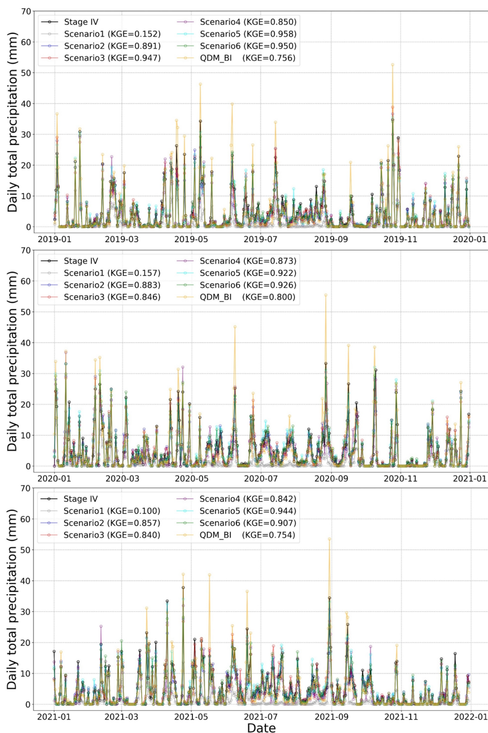
Figure 5. Daily total precipitation during the testing period (2019–2021) from Stage IV, QDM_BI, and the 6 DL experimental runs (Scenario1–Scenario6).
