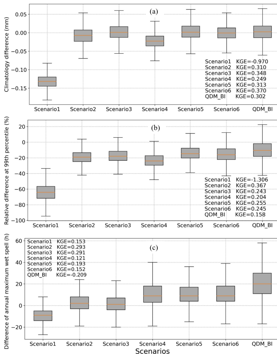
Figure 4. Boxplots showing hourly precipitation estimates minus Stage IV observations based on (a) climatology, (b) extreme at 99 % percentile, and (c) annual maximum wet spell in hours during the testing period (2019–2021). Precipitation estimates are produced from the QDM_BI approach and 6 DL experimental runs (Scenario1–Scenario6).
