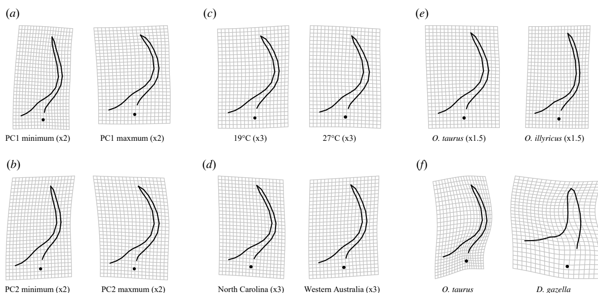
Figure 5. Phenotypic changes associated with FA (PC1 (a) and PC2 (b)), thermal plasticity (c) and evolutionary divergence on different levels for major horn shape (d–f), (d) population divergence in O. taurus , (e) divergence between sister species and (f) divergence between distantly related species. Pictures show deformations relative to the average shape (magnification is indicated).
