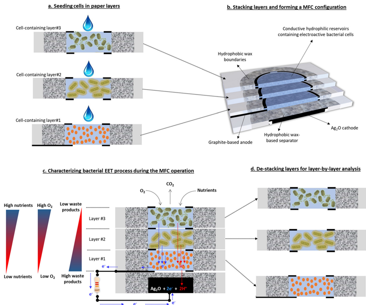
Fig. 1 Schematic diagram of our paper-based biofabrication and characterization platform for 3-D multispecies electroactive biofilm models. After individual paper layers are inoculated with electroactive bacteria as scaffolds (a), they are stacked to form a layered 3-D multispecies biofilm model (b). Mass transport of nutrients and oxygen into the 3-D system are regulated to explore the bacterial EET process and current generation within controlled biofilms (c). De-stacking the multi-layered biofilm construct allow layer-by-layer analysis for pH distribution and cellular viability (d).
