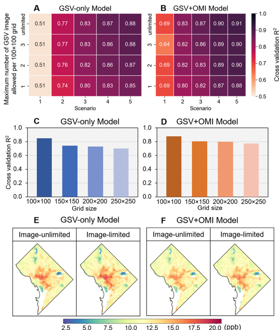
Figure 3. Results of sensitivity analyses among image sampling strategies. Panels (A) and (B) show model results among all scenarios, with varying maximum number of GSV images per 100 m \times 100 m sampling grid. Panels (C) and (D) show model results in scenario 5 with varying grid sizes. Each grid cell is allowed one GSV image for sampling. Panels (E) and (F) show model predictions for Washington DC in 2019 using image-unlimited models and image-limited models, with maximum one GSV image per 100 m \times 100 m grid.
