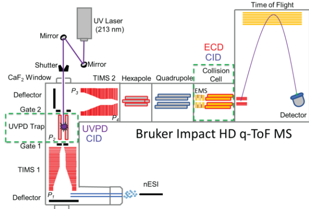
Figure 1. Schematic of the nESI-UVPD-TIMS-q-ECD-ToF MS/MS instrument. The green dashed lines represent the possibility for MS/MS events, for which UVPD/CID and ECD/CID can be performed in the UVPD trap and collision cell, respectively.
