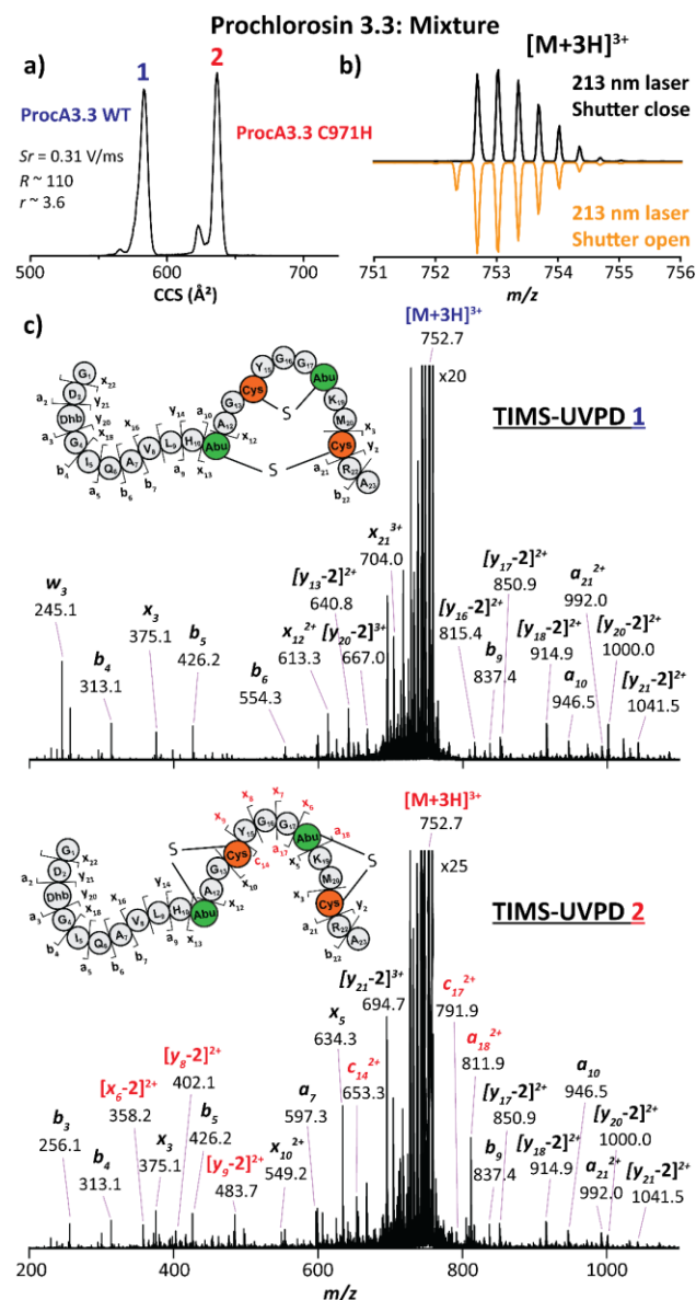
Figure 2. TIMS-UVPD-ToF MS analysis of the selected [M + 3H]^{3+} species of ProcA3.3 WT (blue) and ProcA3.3 C971H (red) isomeric lanthipeptides ( m/z 752.7). (a) TIMS profile in a binary mixture, (b) isotopic pattern distribution of the precursor ion produced with UV laser shutter close (top) and shutter on (bottom). (c) Ion mobility UVPD-IMS/MS spectra. Typical non-overlapping ring pattern specific product ions are highlighted in red. The residues involved in the thioether cross-link are colored in orange (former Cys) and green (former Thr), respectively.
