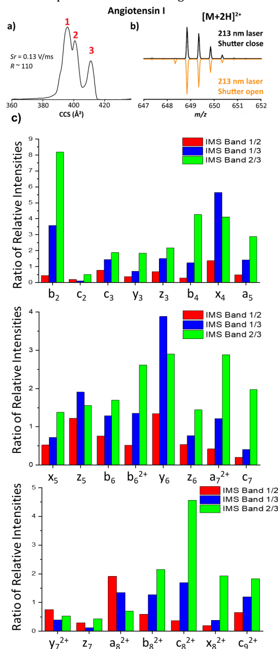
Figure 4. TIMS-UPVD-ToF MS analysis of the selected [M + 2H]^{2+} species of angiotensin I ( m/z 648.9). (a) TIMS profile, (b) isotopic pattern distribution of the precursor ion produced with UV laser shutter close (top) and with shutter open (bottom) and (c) ratio of the relative intensities per IMS band 1-3 (data shown for variations larger than \pm 0.20 , see
