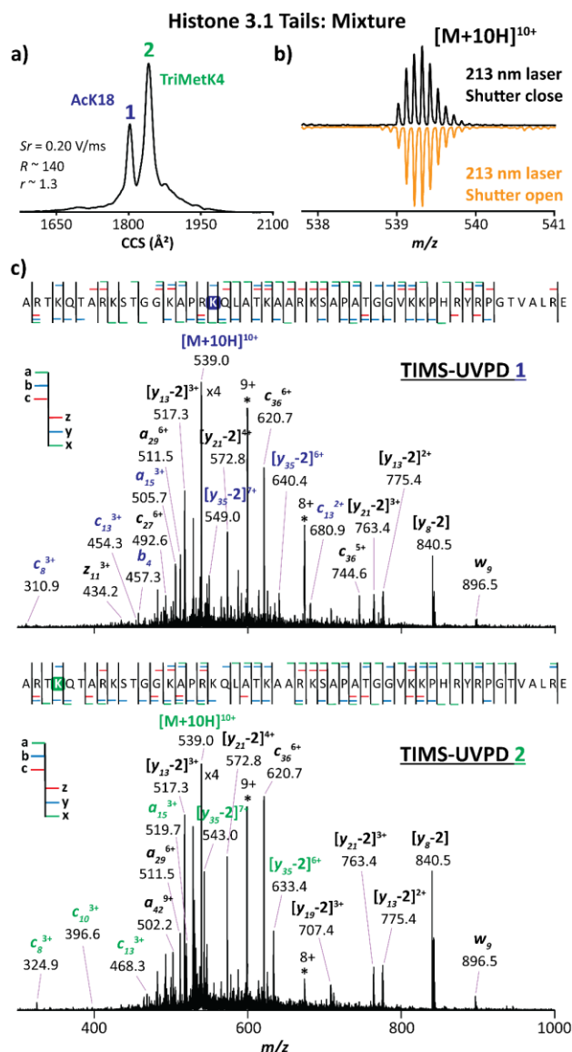
Figure 3. TIMS-UPVD-ToF MS analysis of the selected [M + 10]^{10+} species of K18Ac (blue) and K4Me3 (green) isobaric histone tails ( m/z 539.0). (a) TIMS profile in a binary mixture, (b) isotopic pattern distribution of the precursor ion produced with UV laser shutter close (top) and with shutter open (bottom). (c) Ion mobility UVPD-IMS/MS spectra. The fragments comprising the PTM are highlighted in blue and green for K18Ac and K4Me3, respectively.
