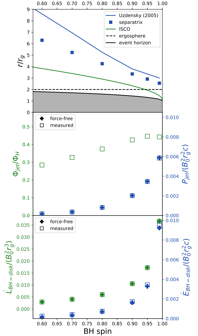
Fig. 5. Reduced quantities as a function of the BH spin. Top panel: ISCO (solid green line), event horizon (solid black line), and ergosphere at the equator (dashed black line) as a function of the BH spin. The blue line indicates the approximate location of the footpoint of the separatrix found by Uzdensky (2005), and the blue squares are the values measured in our simulations. Middle panel: magnetic flux \Phi_{\text{jet}} of the open magnetic field lines threading the event horizon (green, left axis). In blue (right axis) are the jet electromagnetic powers measured (squares) and predicted by Tchekhovskoy et al. (2011) (crosses). Bottom panel: angular momentum (left axis) and energy (right axis) transferred from the BH to the disk per unit time, with and without the force-free approximation (crosses and squares).
