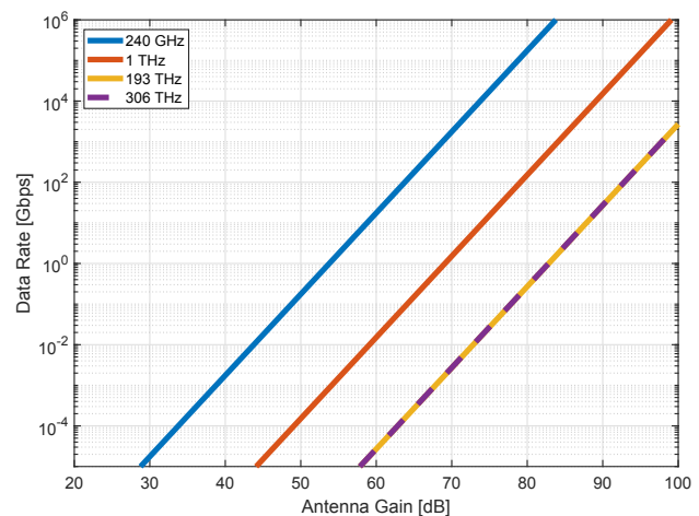
Fig. 3: Estimated data rates for cross-links between satellites in LEO orbit 100 km apart. The calculations utilize transmit power from Table I, noise figure of 8 dB, a bit error rate of 10^{-6} and 16-QAM modulation.
